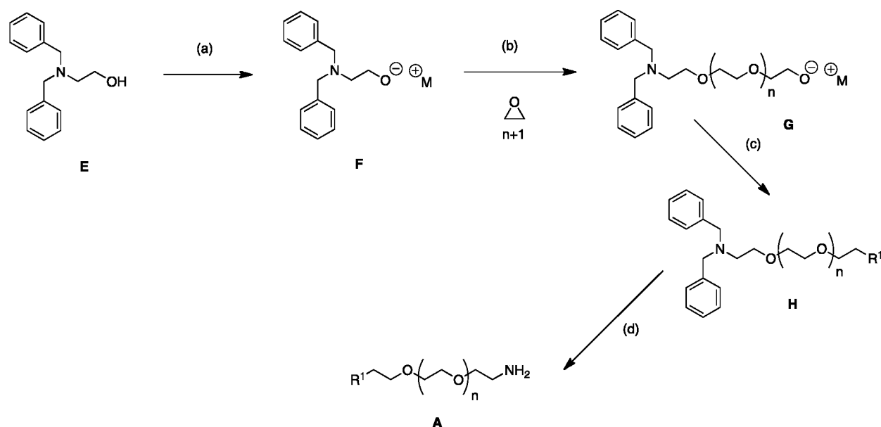
Scheme 4
