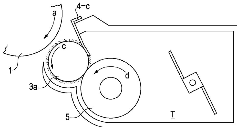
FIG. 11 PRIOR ART
