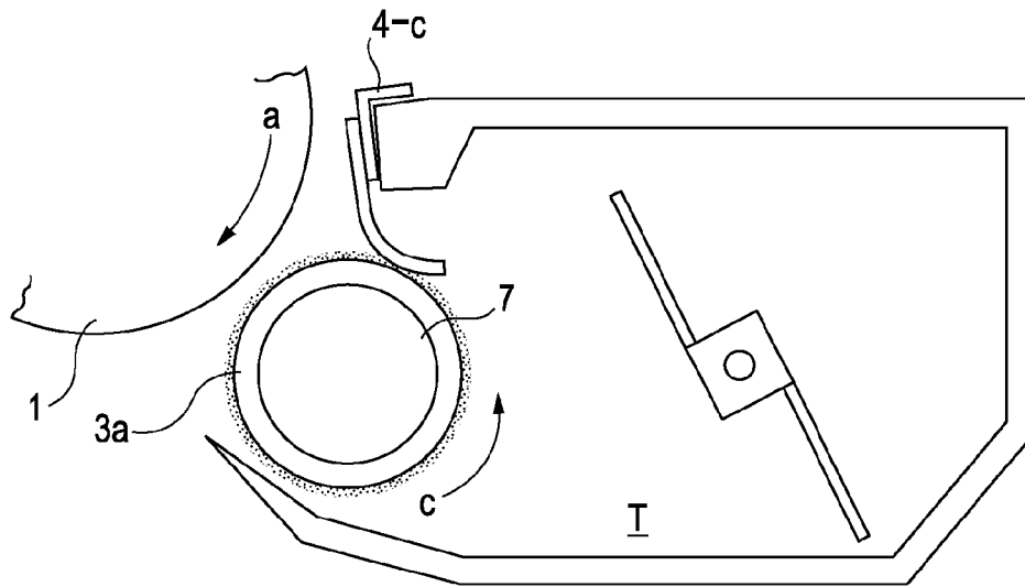
FIG. 12 PRIOR ART
