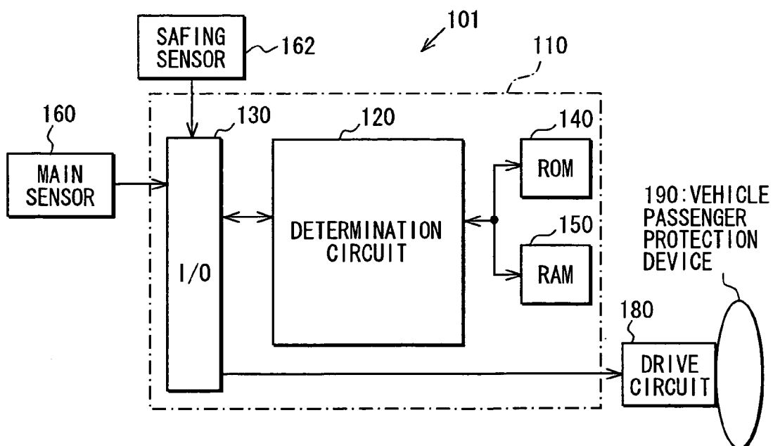
FIG. 11 PRIOR ART
