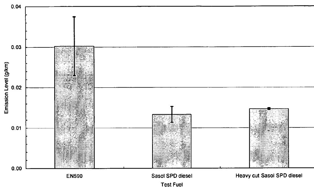
Figure 3 : Composite HC Emissions
