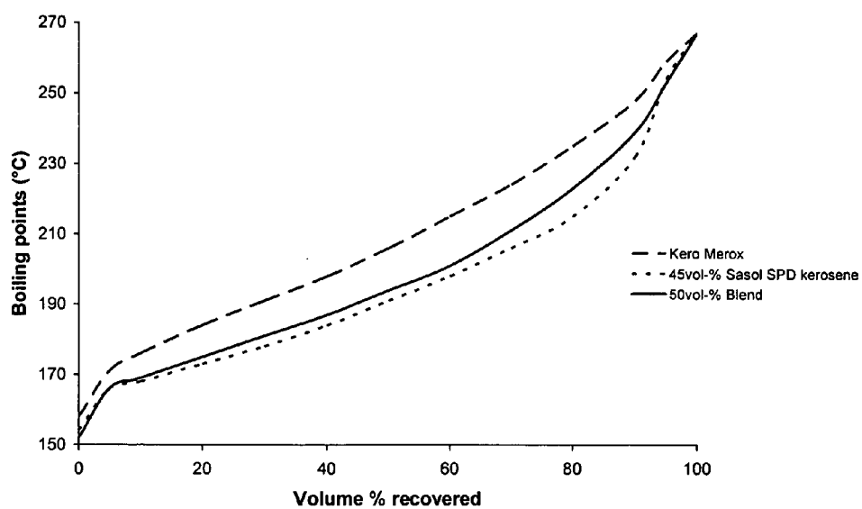
Figure 11: Distillation profiles of sweetened Kero Merox™ kerosene, the 45% Sasol SPD™ kerosene fraction and a 50% blend thereof
