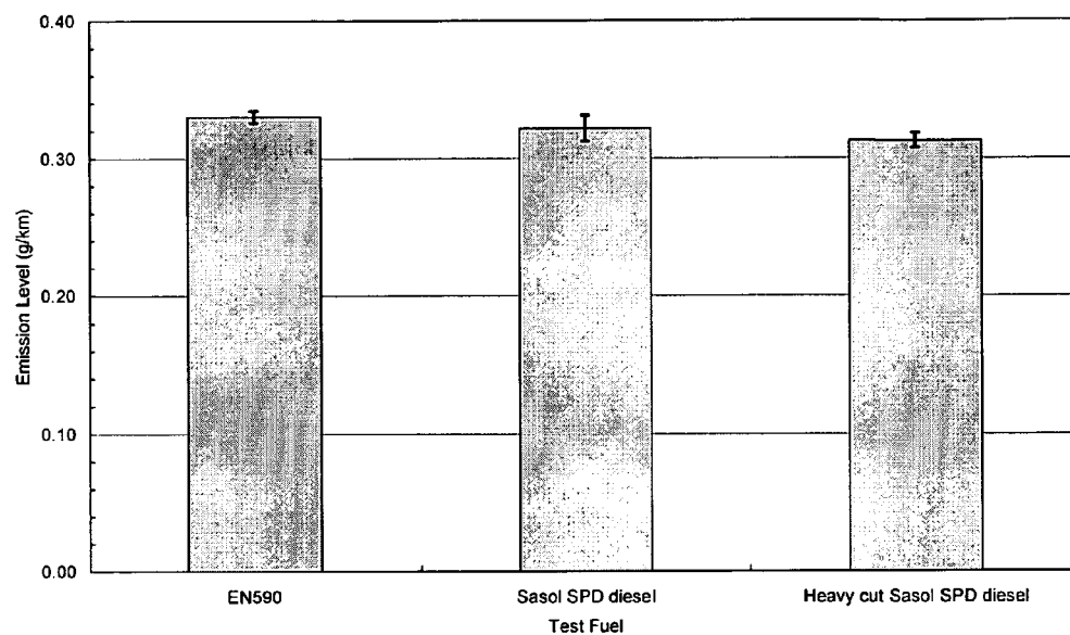
Figure 5 : Composite NOx Emissions
