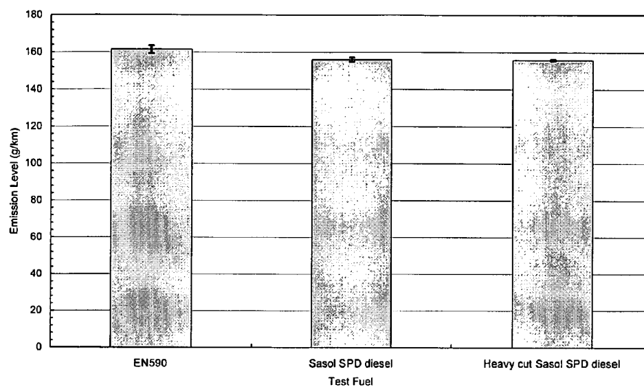
Figure 7 : Composite CO 2 Emissions
