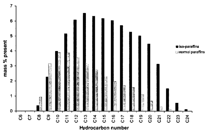
Figure 1: Carbon distribution of Sasol SPD™ diesel
