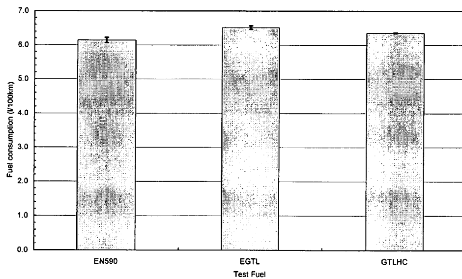
Figure 8 : Fuel Consumption
