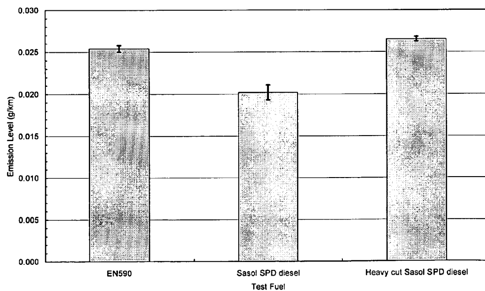
Figure 6 : Composite PM Emissions
