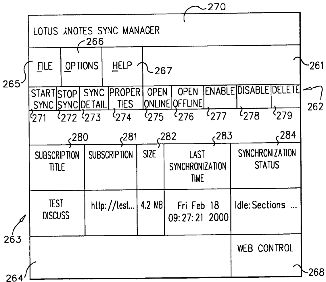
LOTUS &NOTES SYNC MANAGER INITIAL WINDOW
