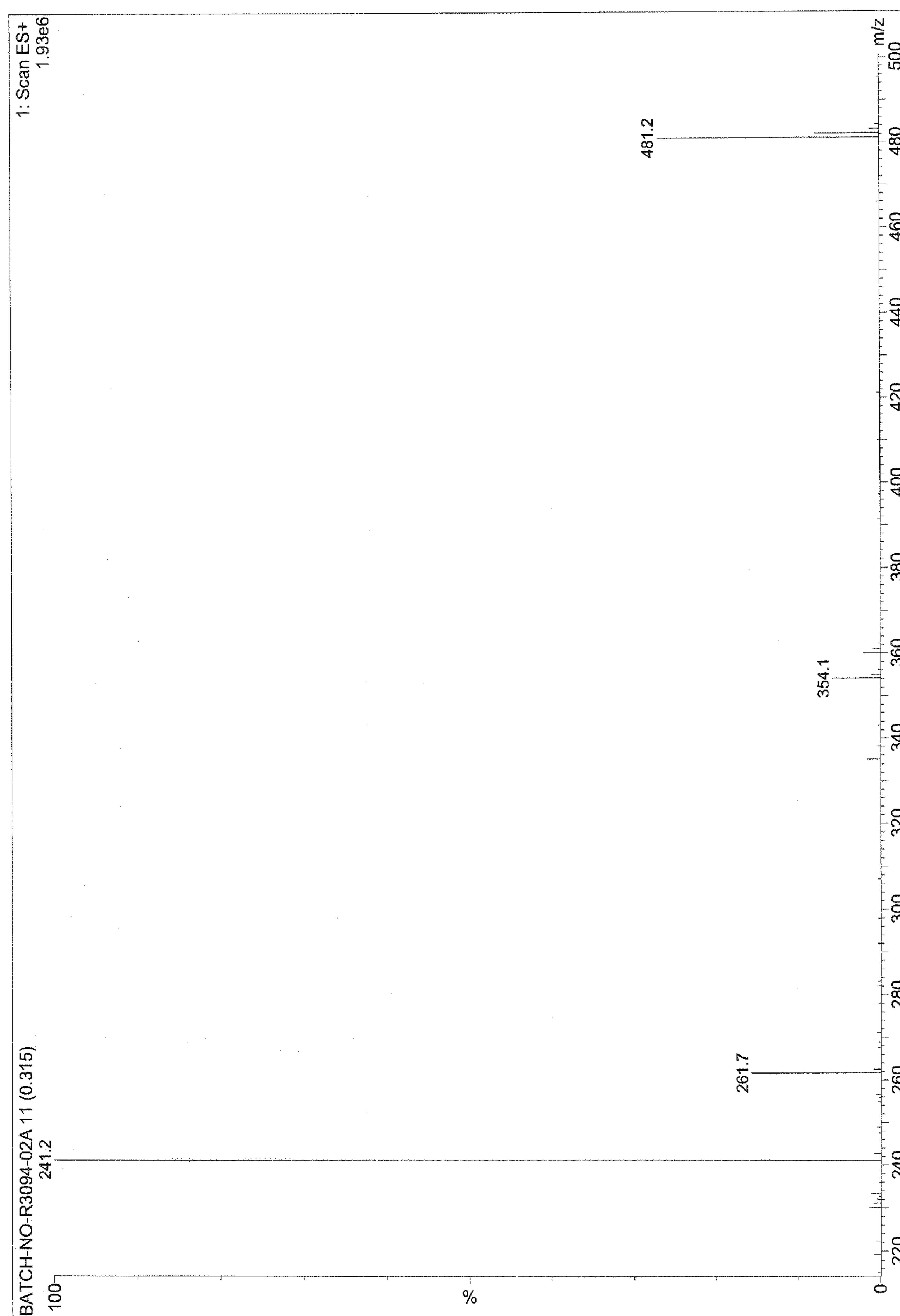
FIGURE 13 Mass Spectrum of the compound A
