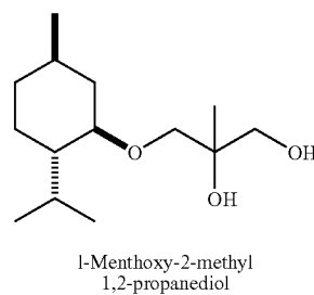
Cooling Agent 10
