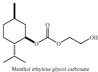
Menthol ethylene glycol carbonate
