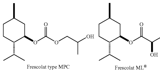
Frescolat type MPC
