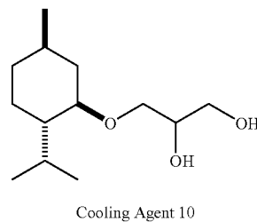
Cooling Agent 10
