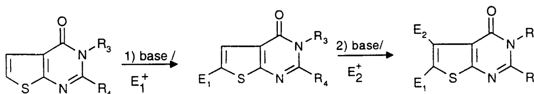
Scheme 2 : Synthesis of special heterocycles
