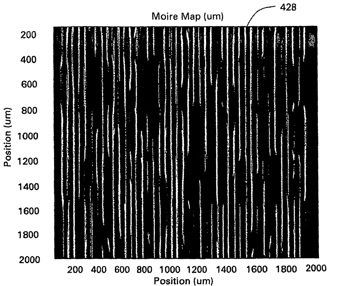
Moire Map of FIG. 26 Against a 44 um Pitch Reference Prism Array
