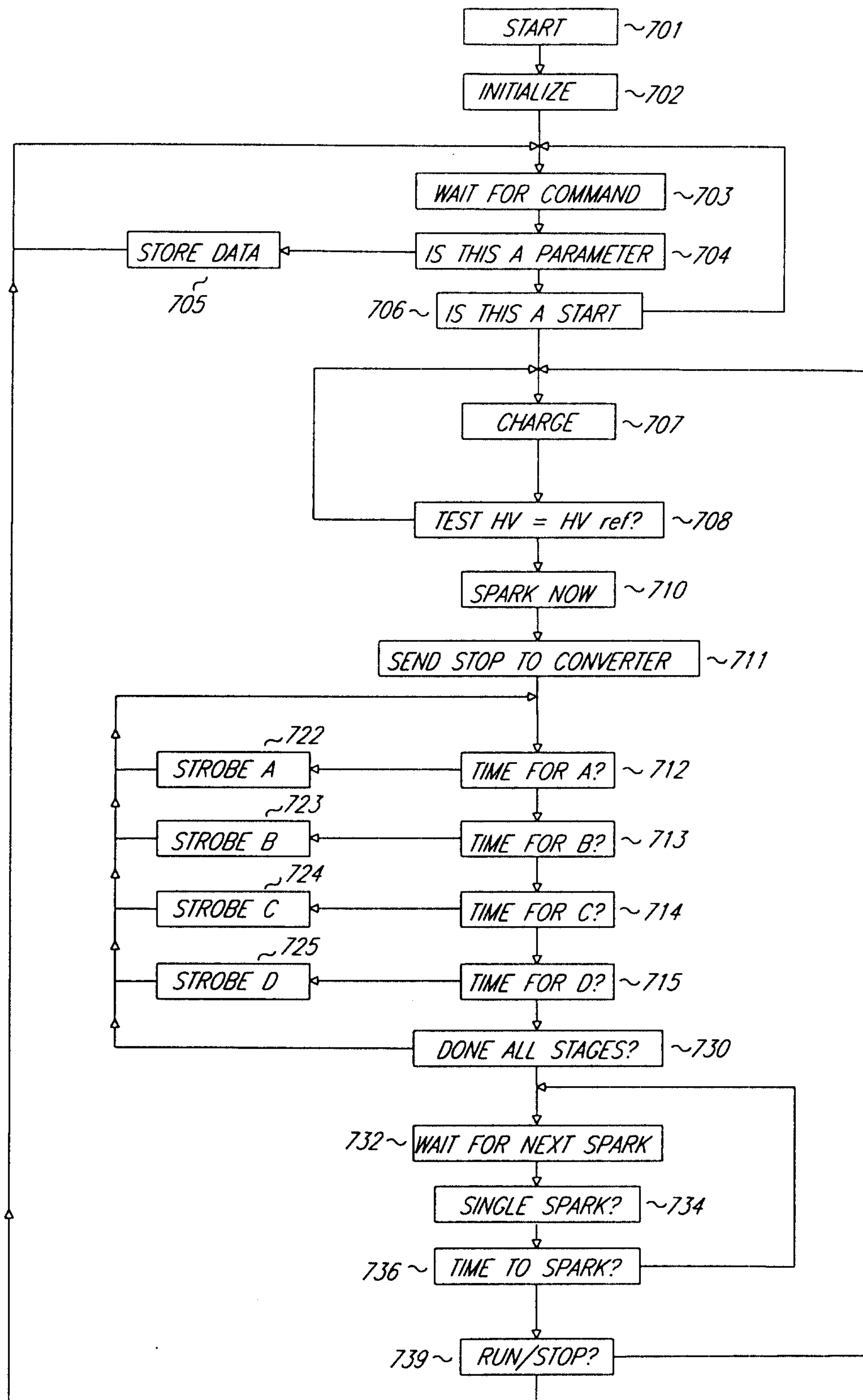
FIGURE 7 FLOWCHART
