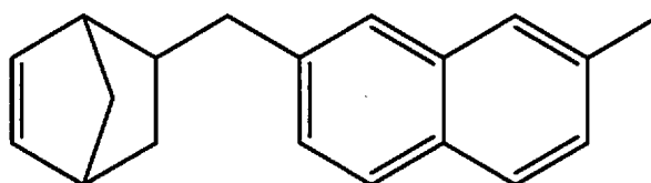
2-(bicyclo[2.2.1]hept-5-en-2-ylmethyl)-7-methylnaphthalene;
