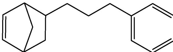
5-(3-phenylpropyl)bicyclo[2.2.1]hept-2-ene;
