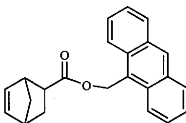
anthracen-9-ylmethyl bicyclo[2.2.1]hept-5-ene-2-carboxylate;
