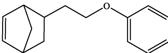
5-(2-phenoxyethyl)bicyclo[2.2.1]hept-2-ene;
