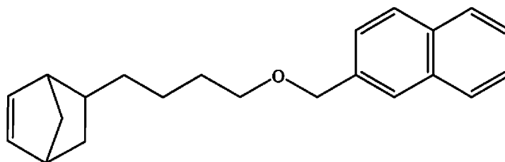
2-((4-(bicyclo[2.2.1]hept-5-en-2-yl)butoxy)methyl)naphthalene;
