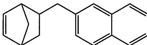
2-(bicyclo[2.2.1]hept-5-en-2-ylmethyl)naphthalene;
