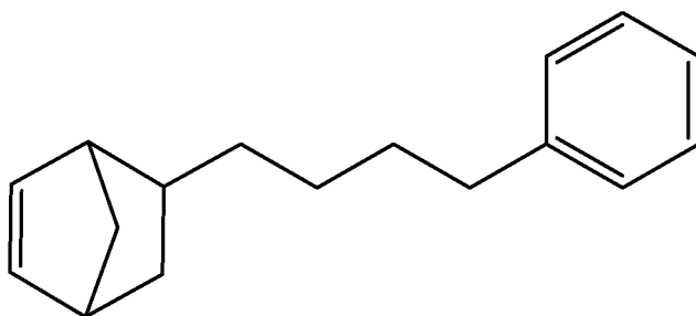
5-(4-phenylbutyl)bicyclo[2.2.1]hept-2-ene;
