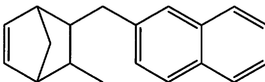
2-((3-methylbicyclo[2.2.1]hept-5-en-2-yl)methyl)naphthalene;
