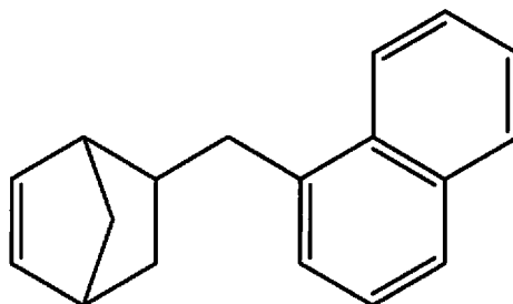
1-(bicyclo[2.2.1]hept-5-en-2-ylmethyl)naphthalene;
