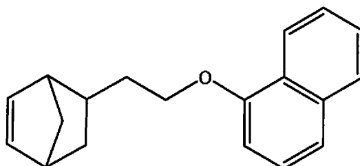
35 40 NBEtO-1-Naphthyl
