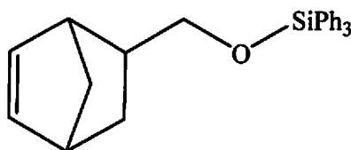
NBMeOSiPh 3
