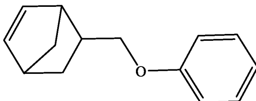
5-((benzyloxy)methyl)bicyclo[2.2.1]hept-2-ene;
