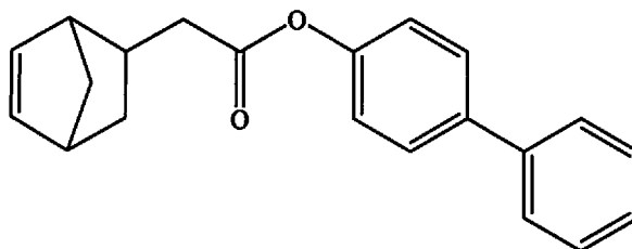
[1,1'-biphenyl]4-yl 2-(bicyclo[2.2.1]hept-5-en-2-yl)acetate;
