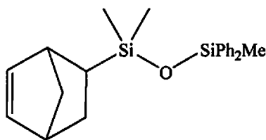
NBSi(CH 3 ) 2 OSiPh 2 CH 3
