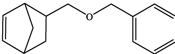
5-((benzyloxy)methyl)bicyclo[2.2.1]hept-2-ene;
