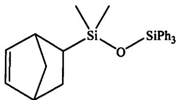
NBSi(CH 3 ) 2 OSiPh 3
