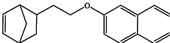
2-(2-(bicyclo[2.2.1]hept-5-en-2-yl)ethoxy)naphthalene (NBEO-2-Naphthyl);
