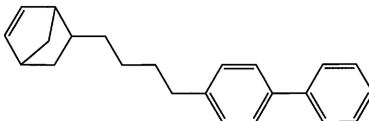
5-(4-([1,1'-biphenyl]-4-yl)butyl)bicyclo[2.2.1]hept-2-ene;
