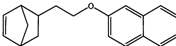
NBEtO-2-Naphthyl
