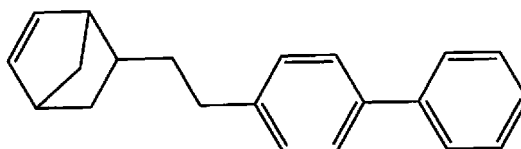
NBEtPhPh
