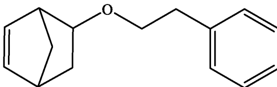
5-(3-phenylpropyl)bicyclo[2.2.1]hept-2-ene;
