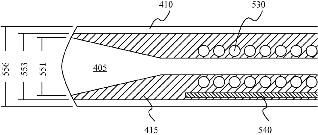
SECTION B-B FIG 5
