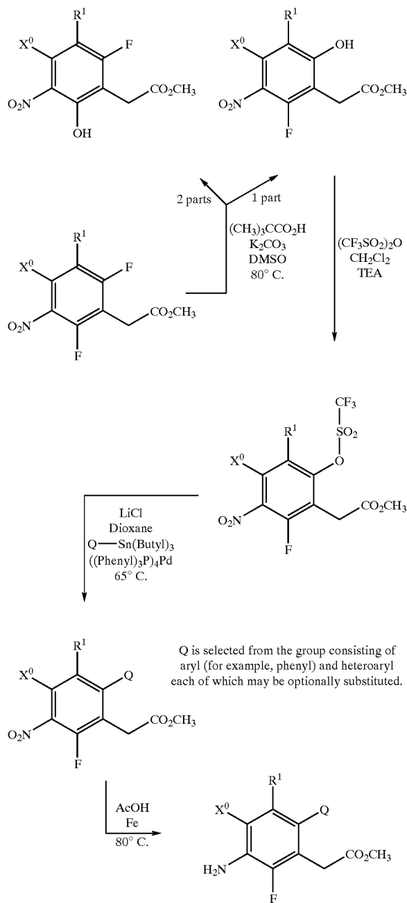
SCHEME 6
