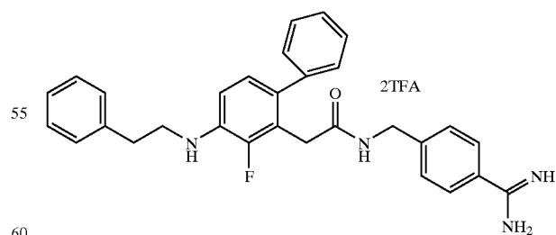
Example 17
