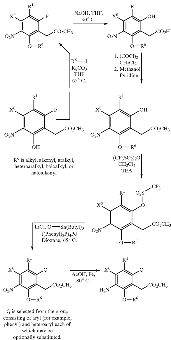
SCHEME 8
