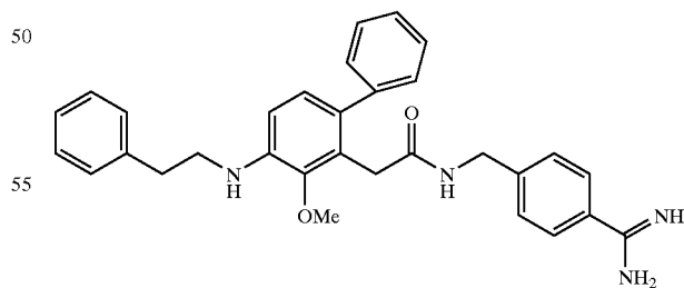
Example 18
