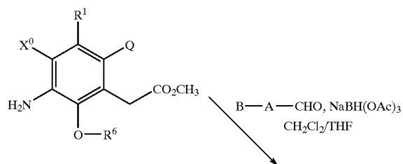
SCHEME 9
