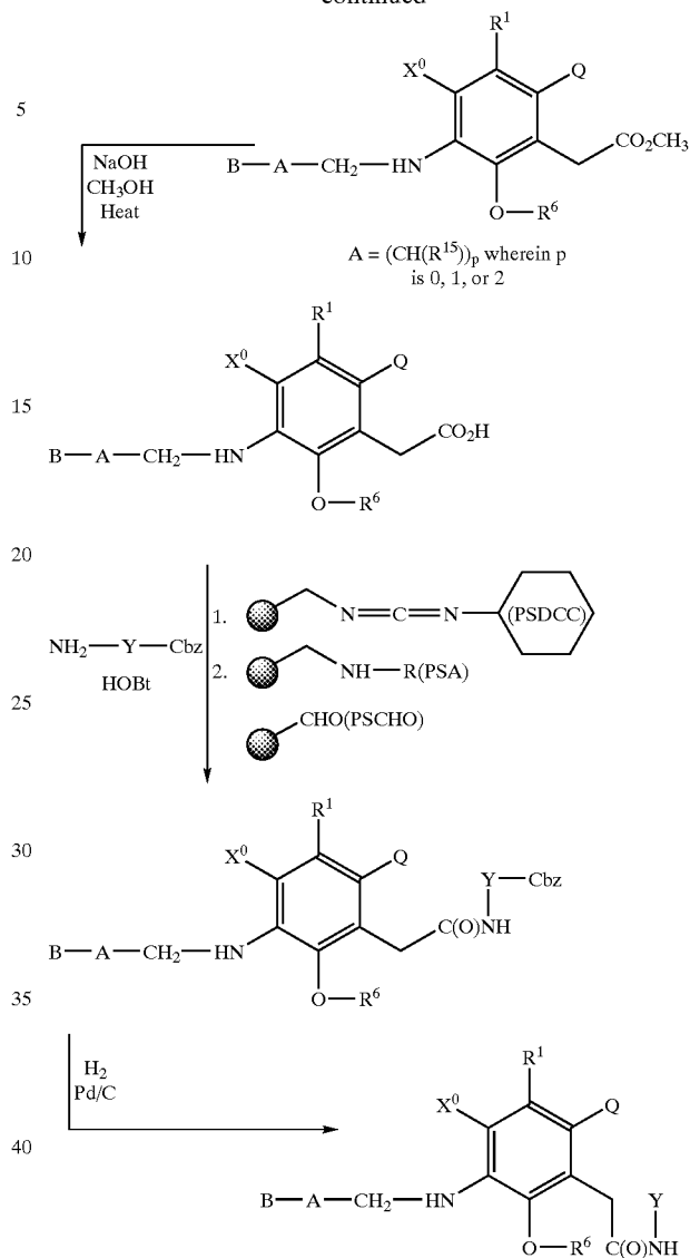
Example 18
