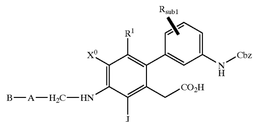
SCHEME 13
