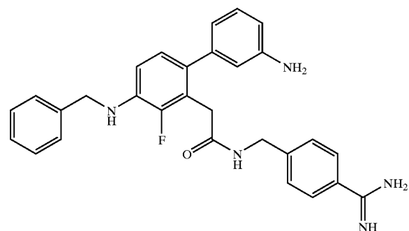
Example 20
