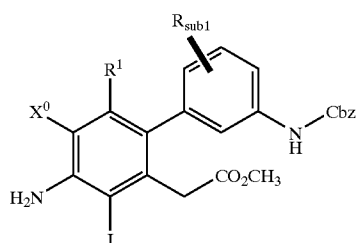
SCHEME 12
