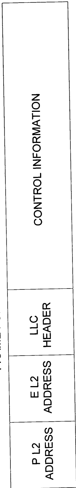
FRAME FORMAT FOR PROXY CONFIGURATION
