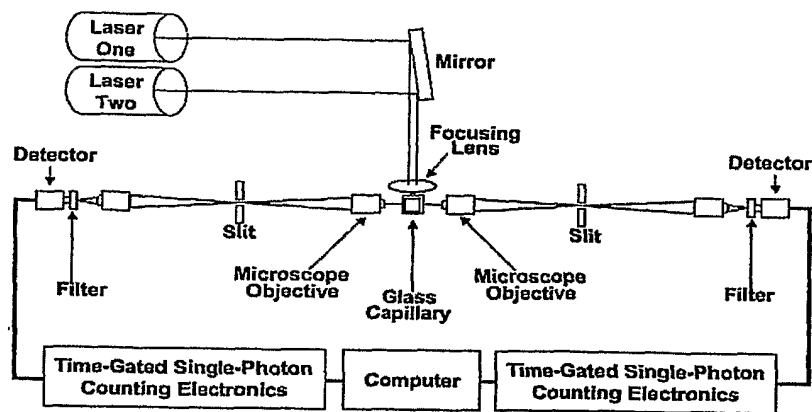
Figure 2 Schematic diagram of the basic apparatus for single molecule detection using laser induced fluorescence.
