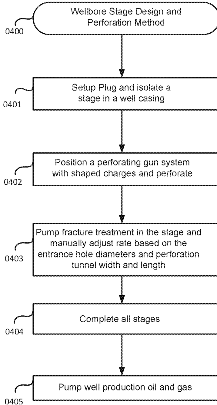
FIG.4 Prior Art
