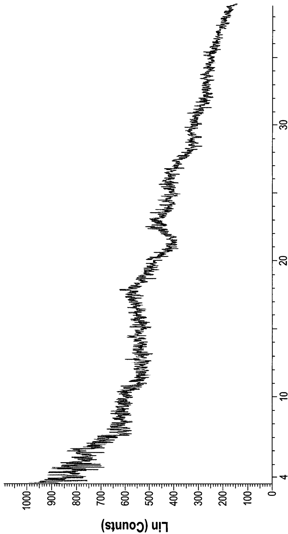
2 - Theta - Scale
