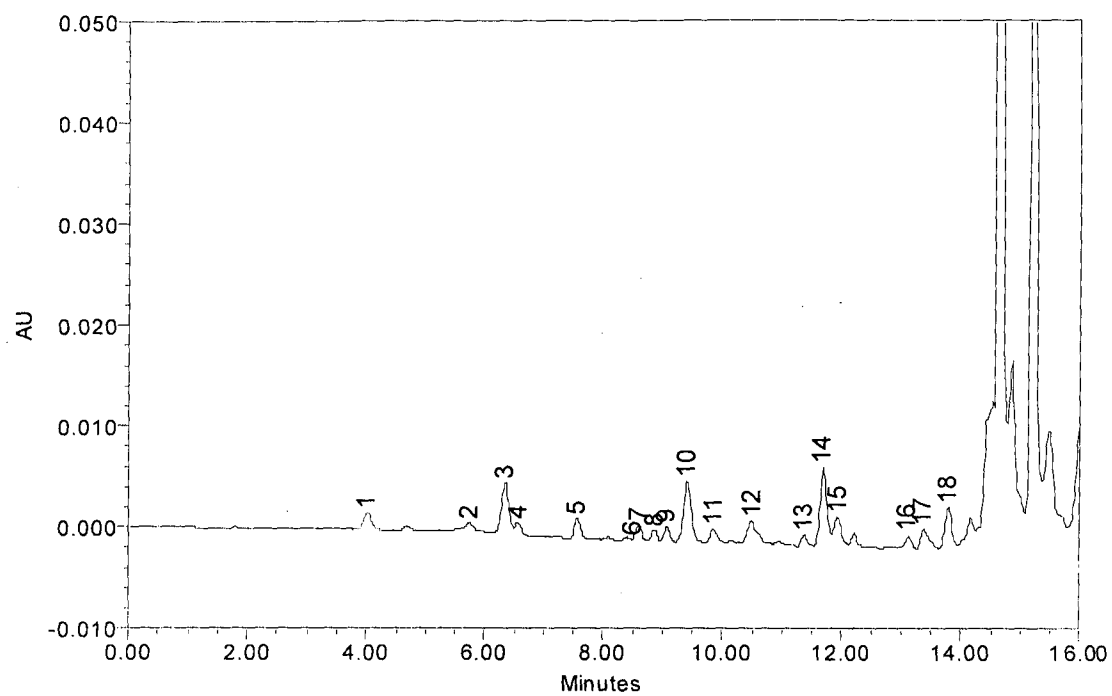
Figure 3a. UPLC chromatogram of standard amino acids
