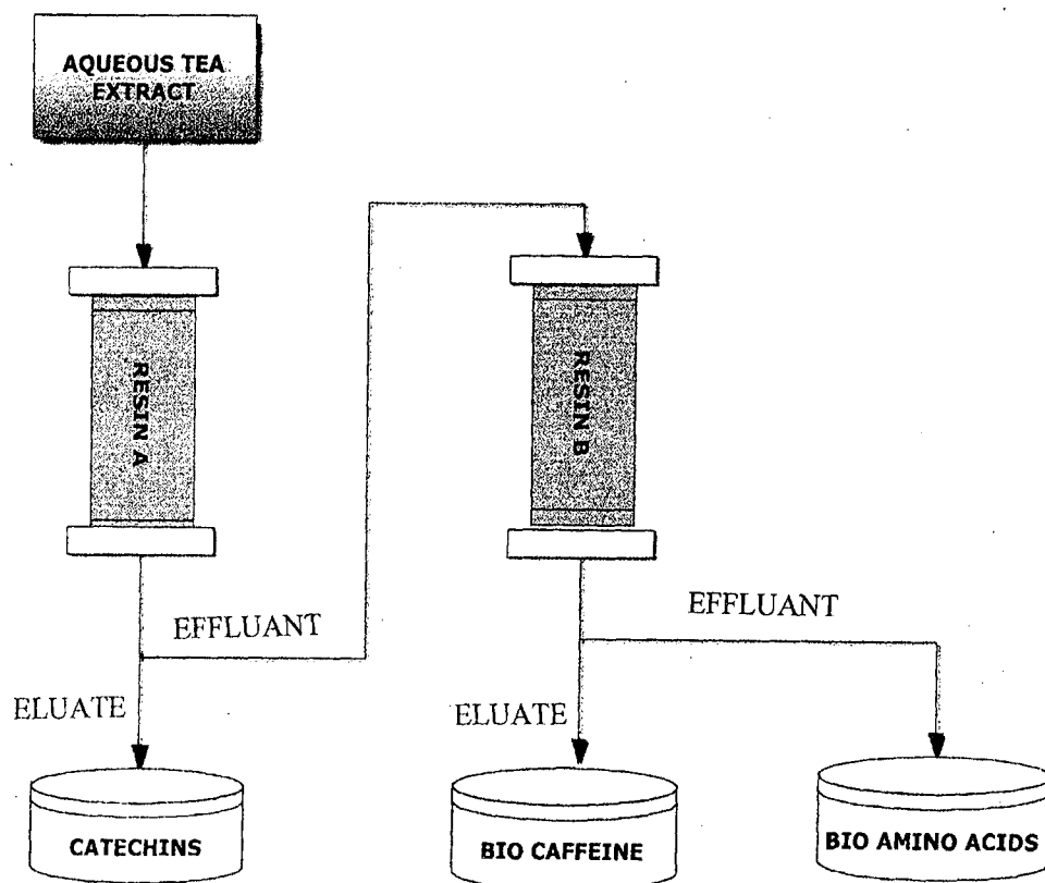
Figure 1- A Schematic Flow Chart Showing Process for Amino Acids Purification
