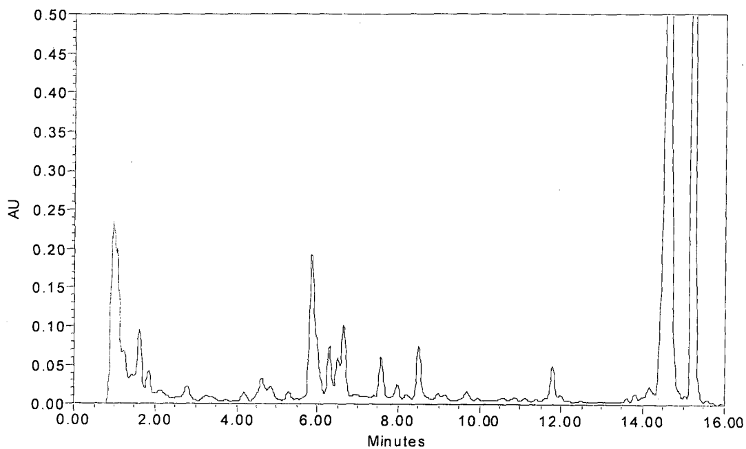
Figure 3c. UPLC Chromatogram of Sesbania bio amino acids
