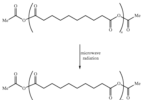
Scheme 5. Polyanhydride Preparation.
