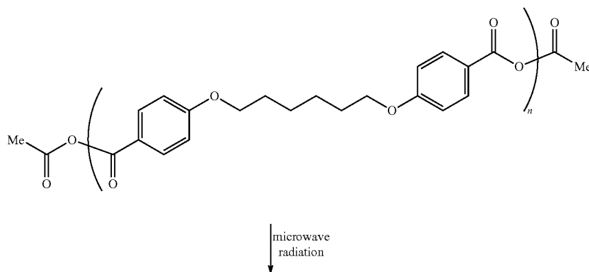
Scheme 6. Polyanhydride Preparation.
