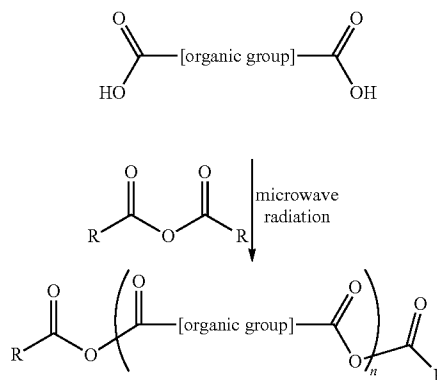
Scheme 1. Prepolymer Preparation.
