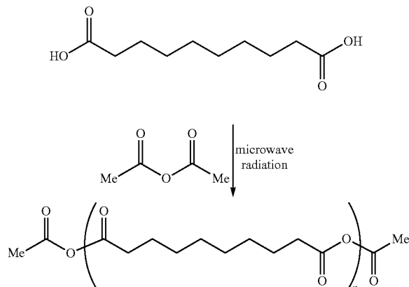
Scheme 2. Prepolymer Preparation.
