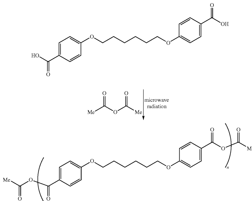
Scheme 3. Prepolymer Preparation.
