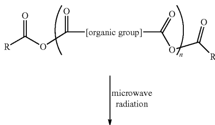
Scheme 4. Polyanhydride Preparation.
