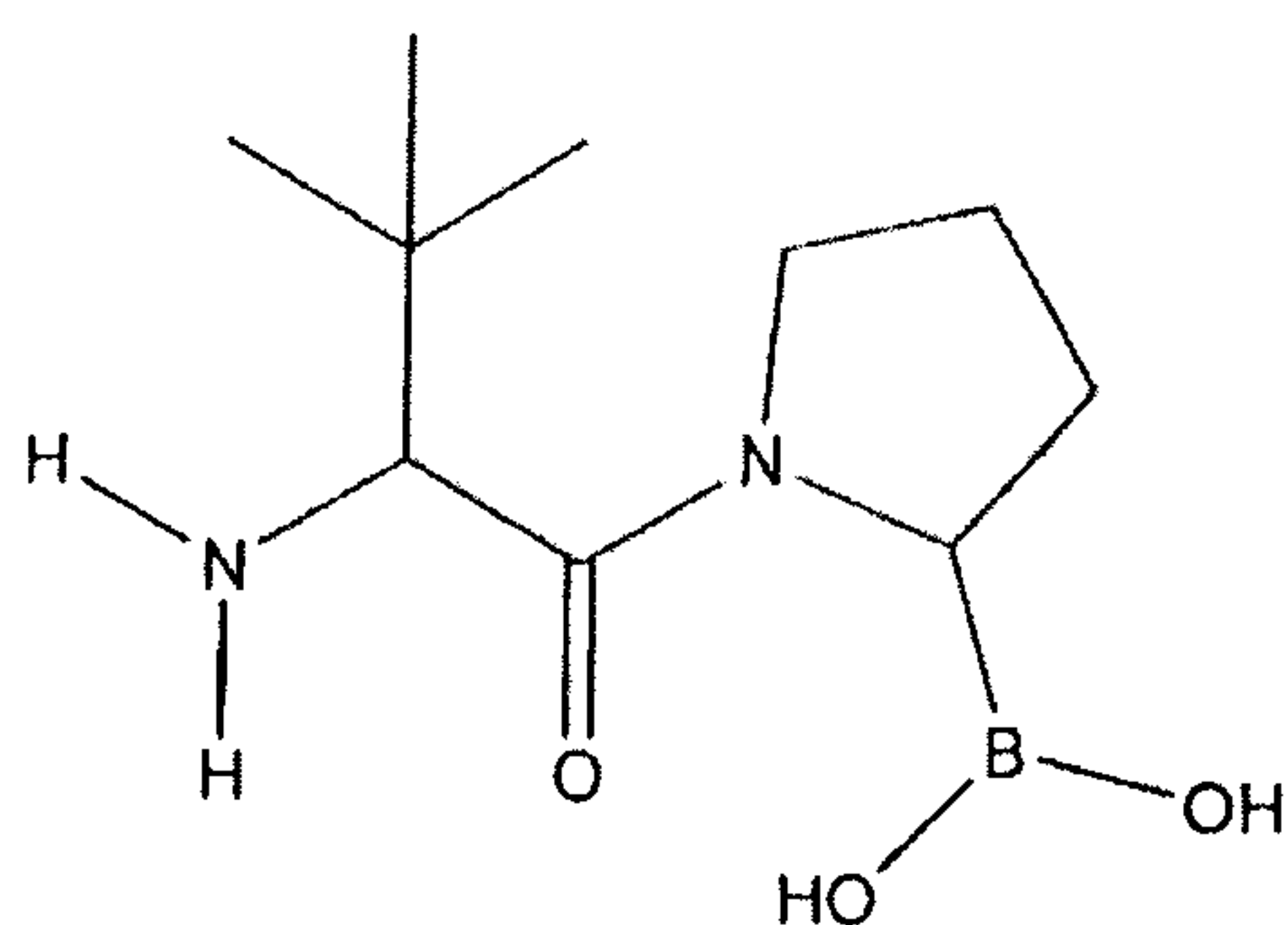
t-Butyl-boroPro
