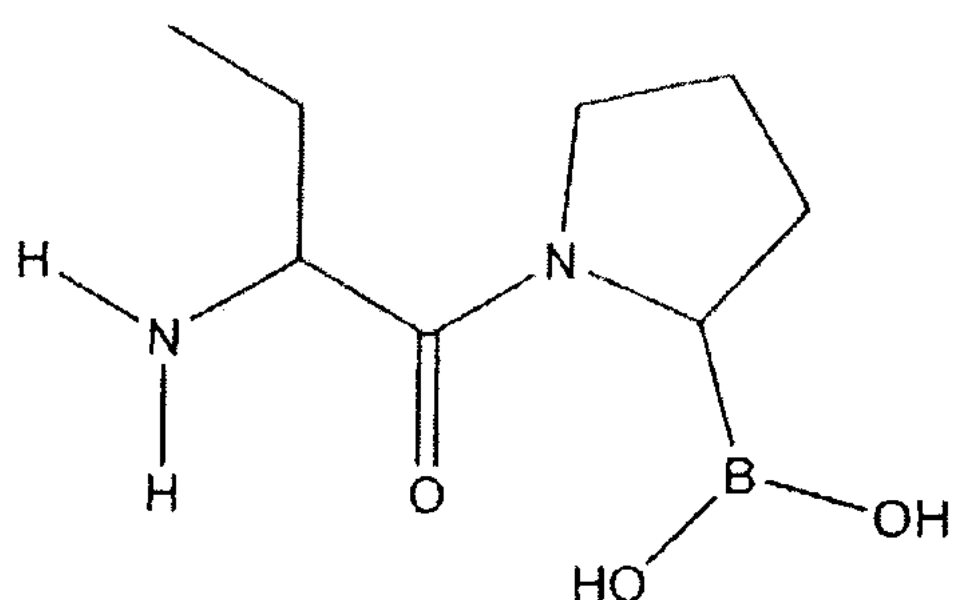
Ethylglycyl-boroPro
