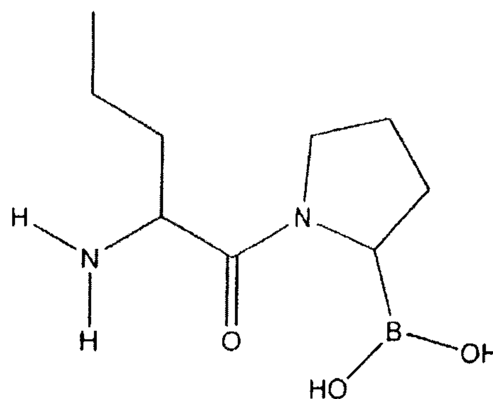
n-Propylglycyl-boroPro
