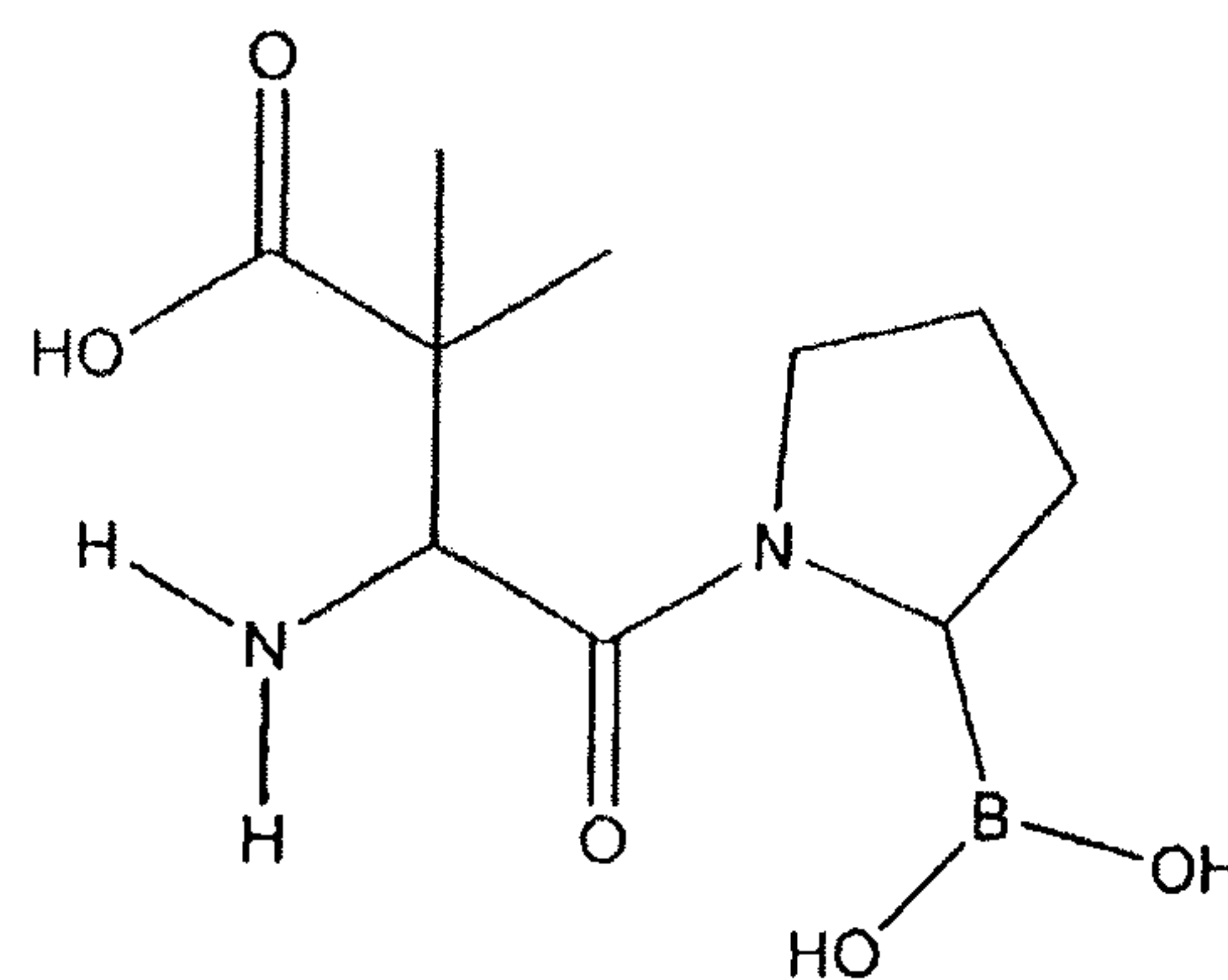
Dimethylglutamyl-boroPro
