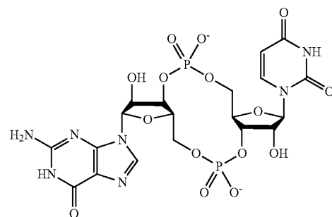
c-GpUp
