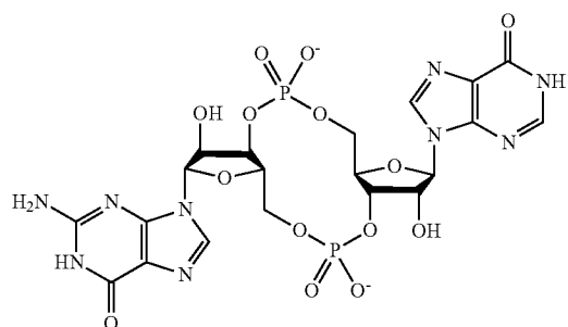
c-GpIp
