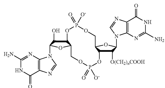
c-GpIp
