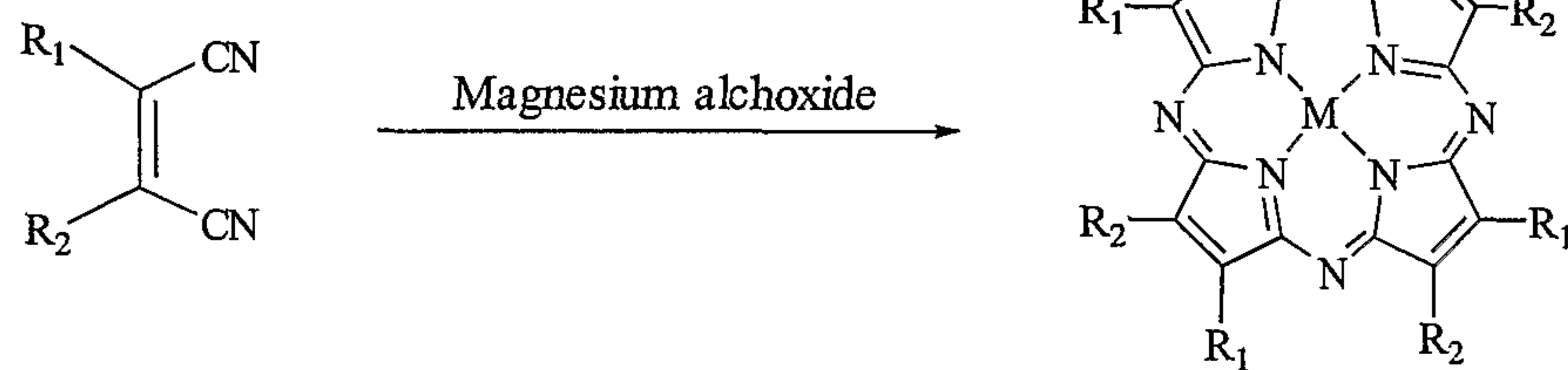
Scheme 3. Azaporphyrin Syntheses
