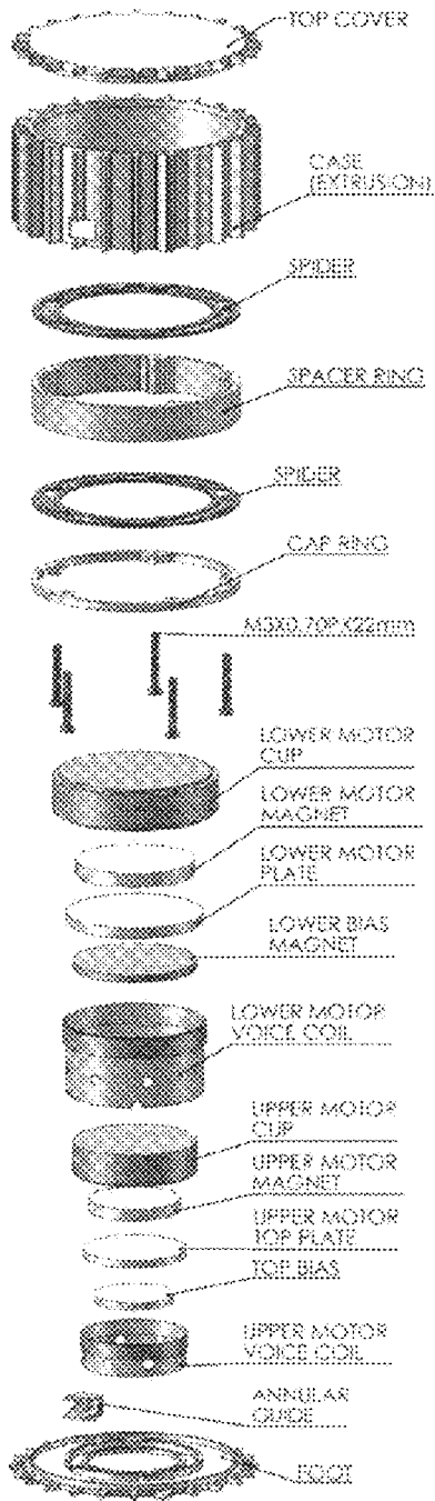
EXPLODED VIEW
