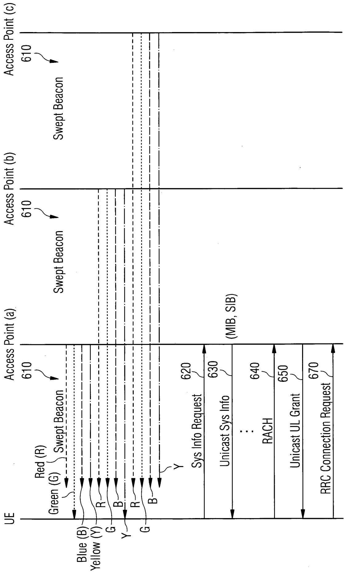
FIG 6 Millimeter wave Access Architecture Cell Selection with Swept Beacon
