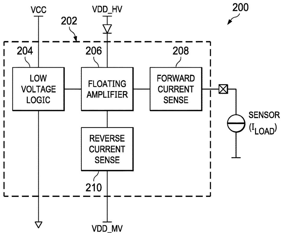
FIG. 2 (PRIOR ART)
