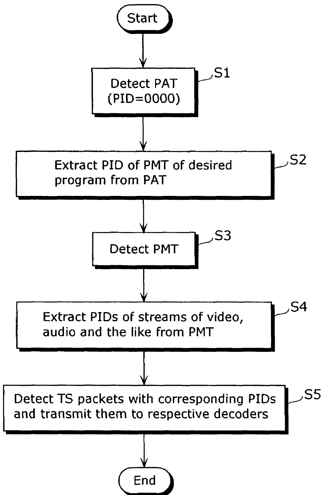
FIG. 3 Prior Art
