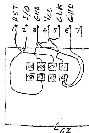
FIG. 6 - Security Card
