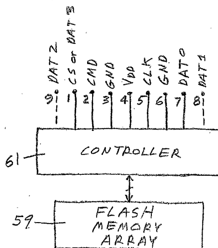
FIG. 5 - Memory Card
