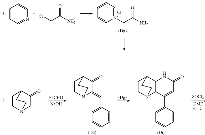
REACTION SCHEME 4
