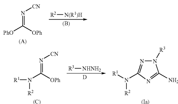
REACTION SCHEME 1
