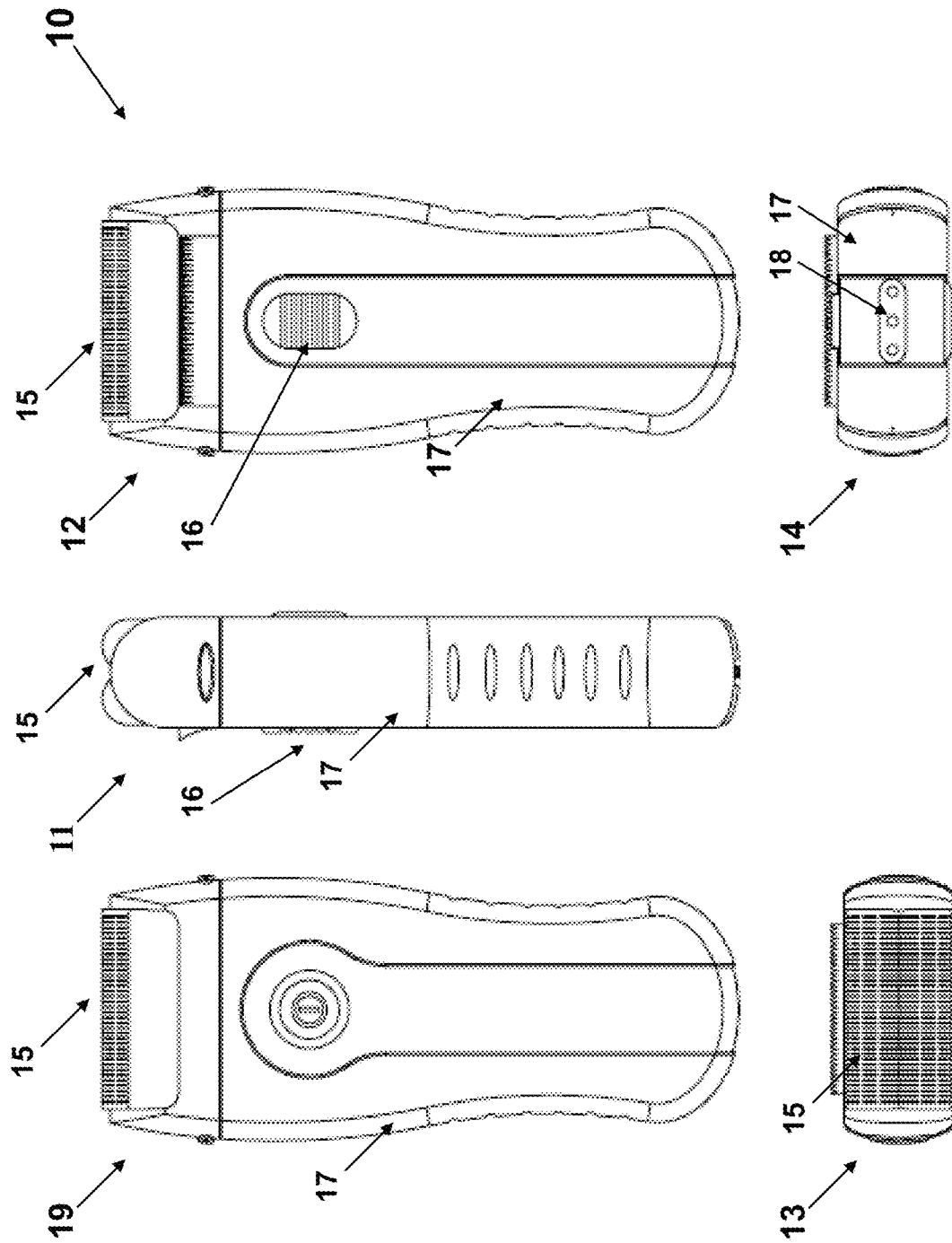
Figure 1 (Prior Art)
