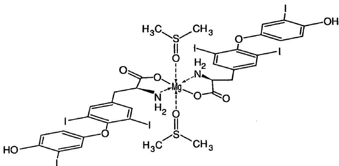
Bis(triiodothyroninato)-bis(dimethylsulfoxide)magnesium
