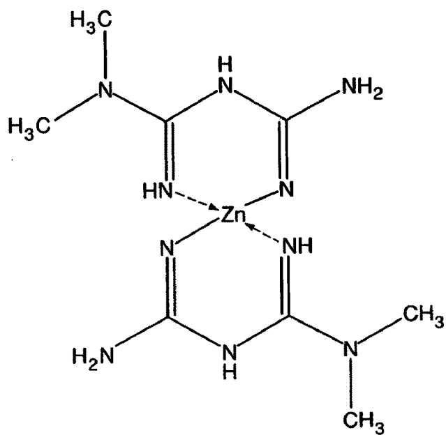
Dimethylbiguanide-zinc complex
