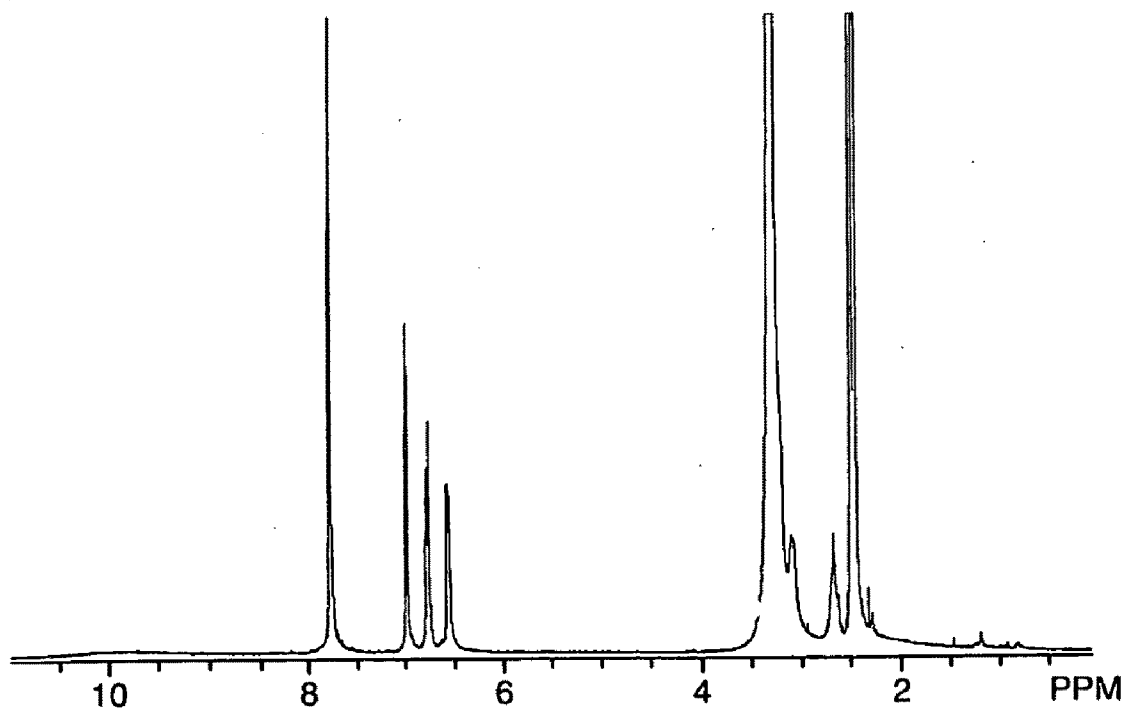
Proton NMR of Bis(triiodothyroninato)- bis(dimethylsulfoxide)magnesium
