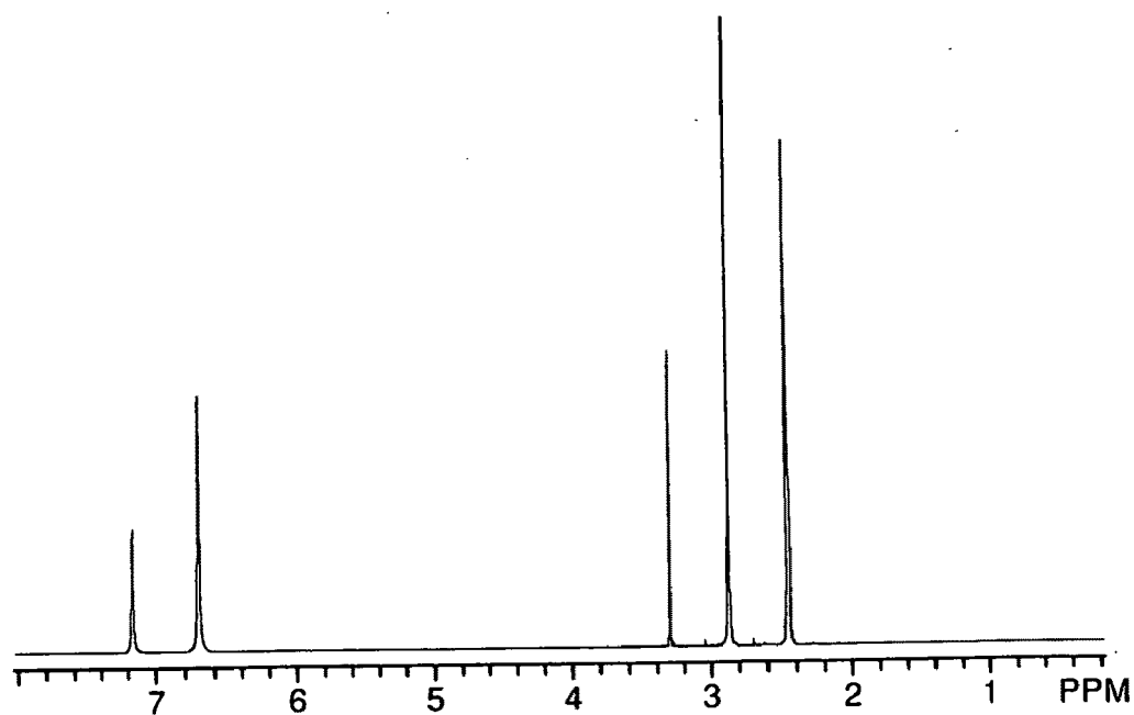
Proton NMR of Dimethylbiguanide
