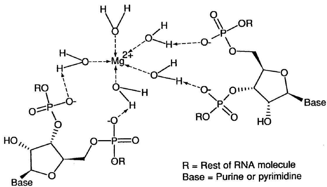
Outer sphere RNA:Magnesium Coordination Complex
