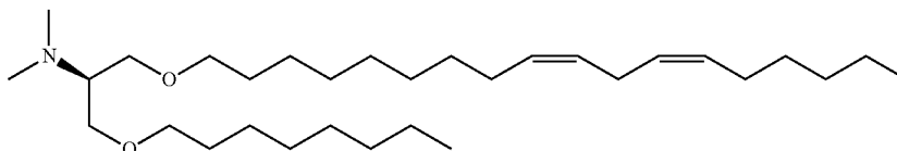
Compound 2
