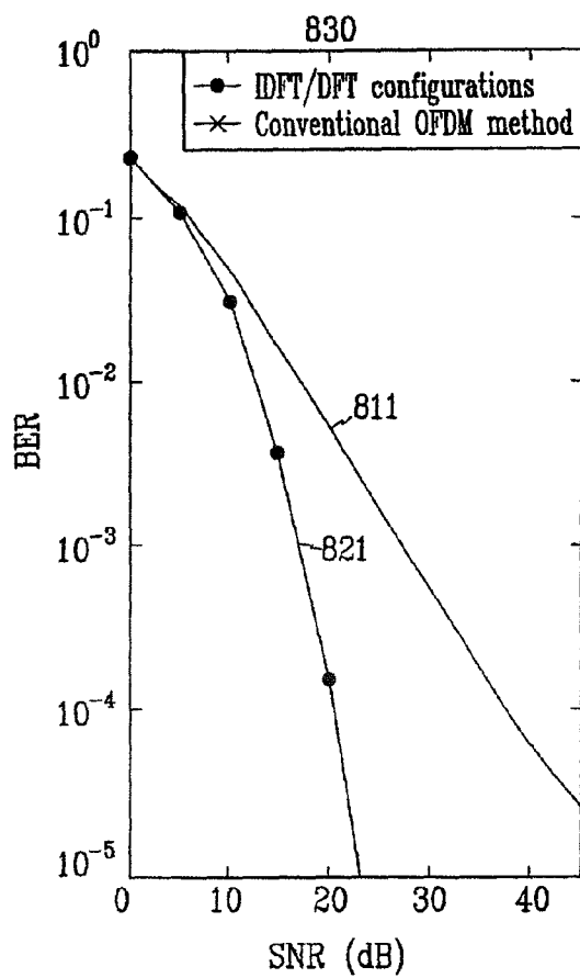
(a) 20Hz
