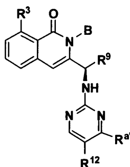
Formula XVIII-A1
