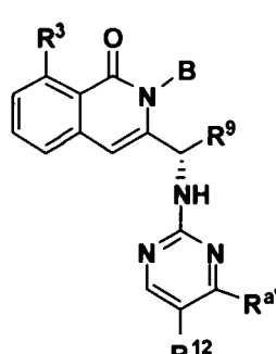
Formula XVIII-A2
