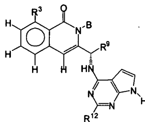
Formula XII-A1
