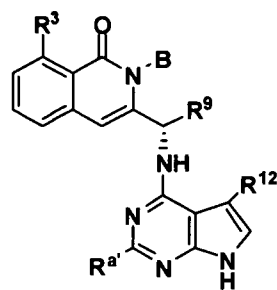
Formula XVI-A2
