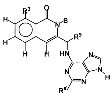
Formula VIII-A
