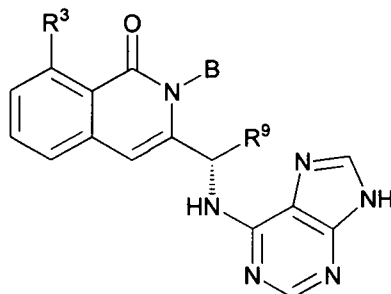
Formula V-A2
