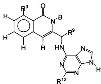
Formula VII-A
