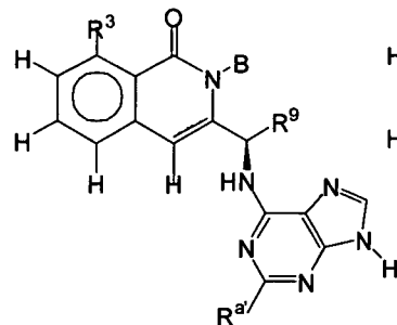
Formula VIII-A1
