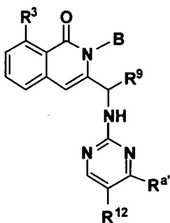
Formula XVIII-A
