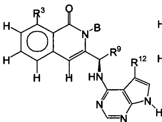
Formula IX-A1
