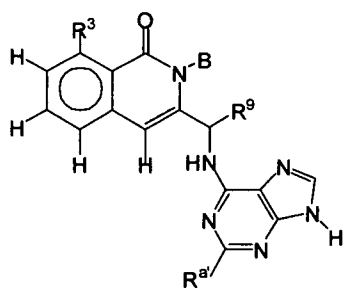
Formula X-A
