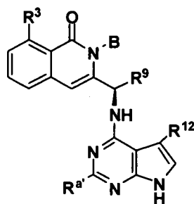
Formula XVI-A1
