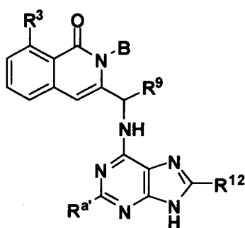
Formula XV-A
