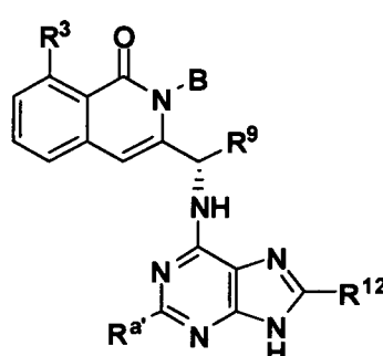
Formula XV-A2
