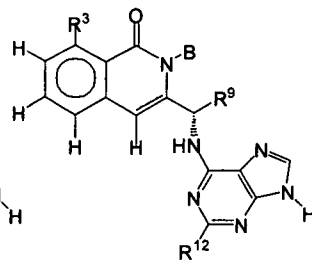
Formula VII-A2
