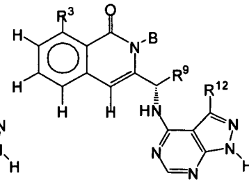
Formula X-A2
