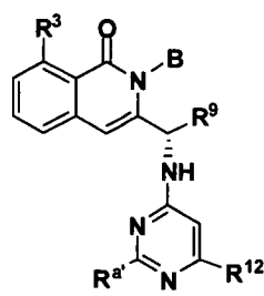
Formula XVII-A2
