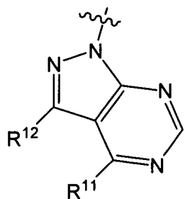
Formula III(a)
