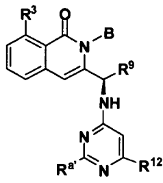
Formula XVII-A1
