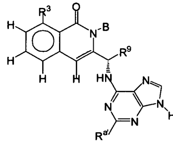
Formula X-A2
