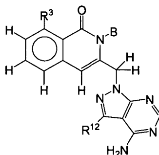
Formula IV-A
