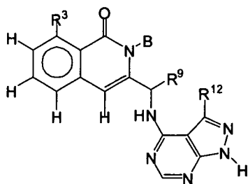
Formula IX-A
