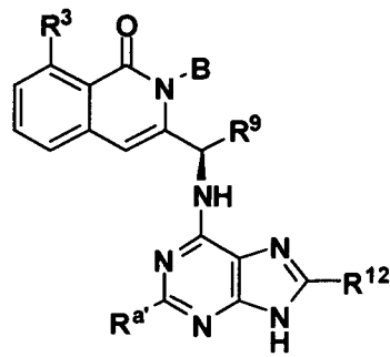
Formula XV-A1
