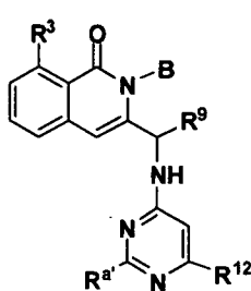
Formula XVII-A
