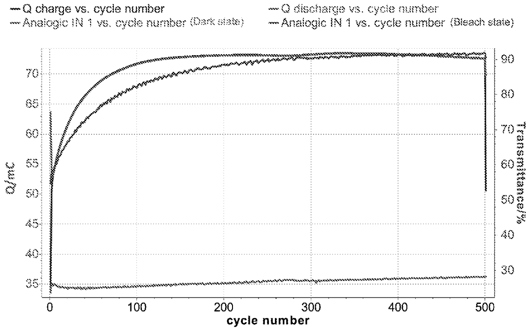
Figure 3 LiNiZrVO x (~200 nm, charge capacity and transmission from CV)
