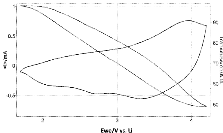
Figure 1 LiNiZrVO x (~80 nm, CV, 50 th cycle)
