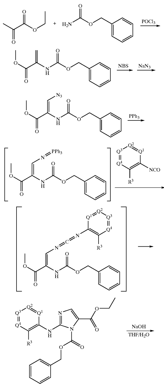
Scheme 9
