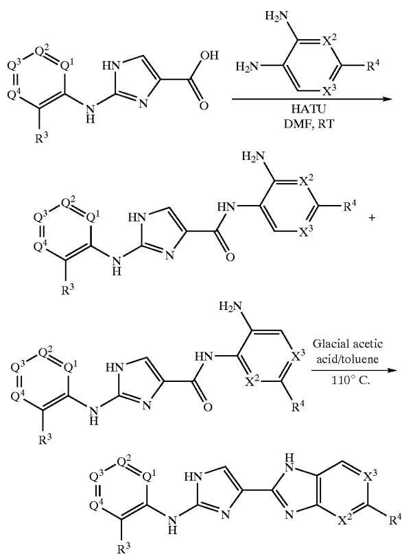
Scheme 12
