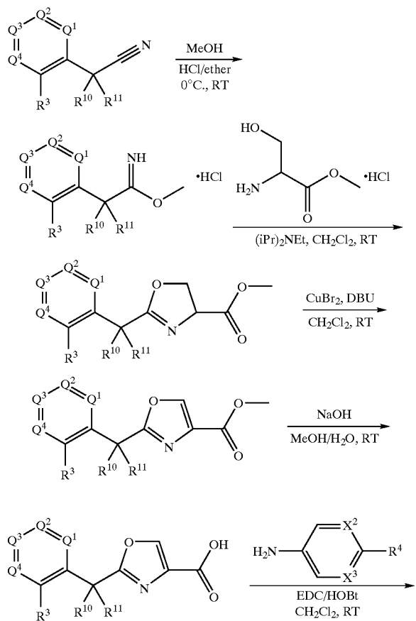
Scheme 14
