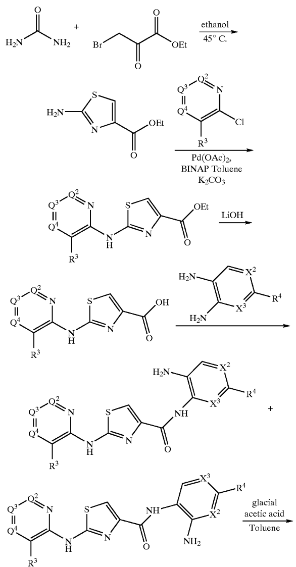
Scheme 8
