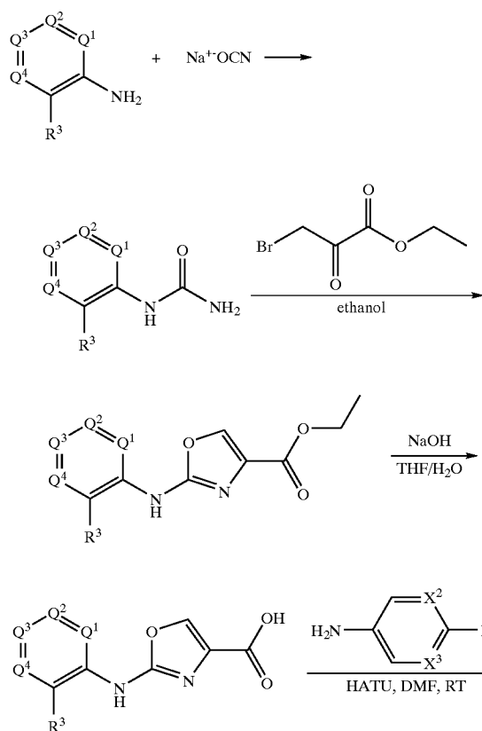
Scheme 10
