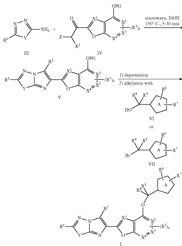
Scheme 1
