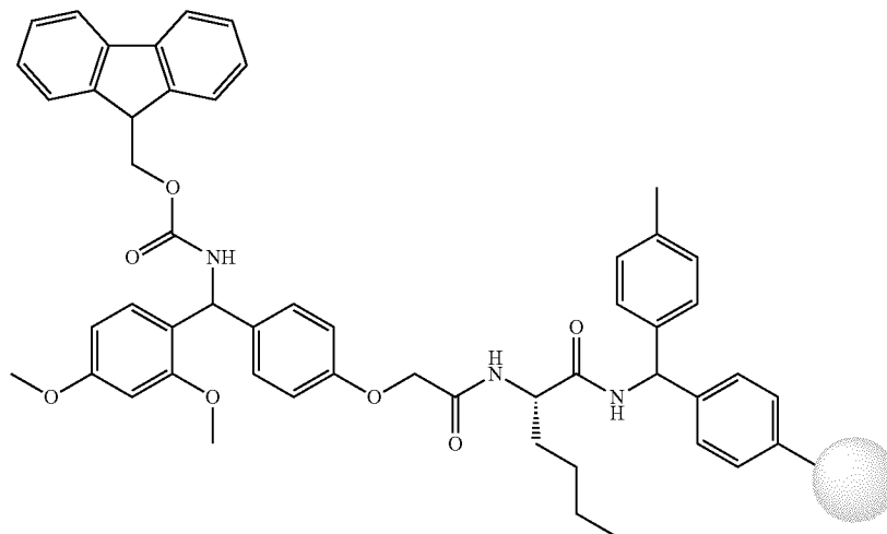
Fmoc-Rink amide MBHA Resin
