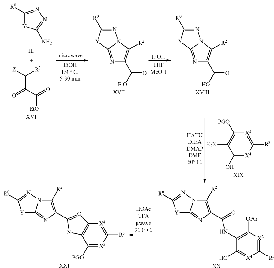
Scheme 4
