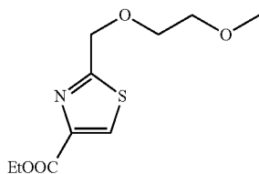
6C. Ethyl 2-((2-methoxyethoxy)methyl)thiazole-4-carboxylate
