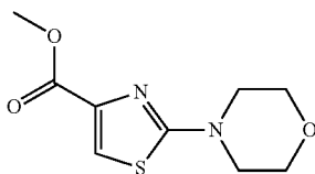
5A. Methyl 2-morpholinothiazole-4-carboxylate
