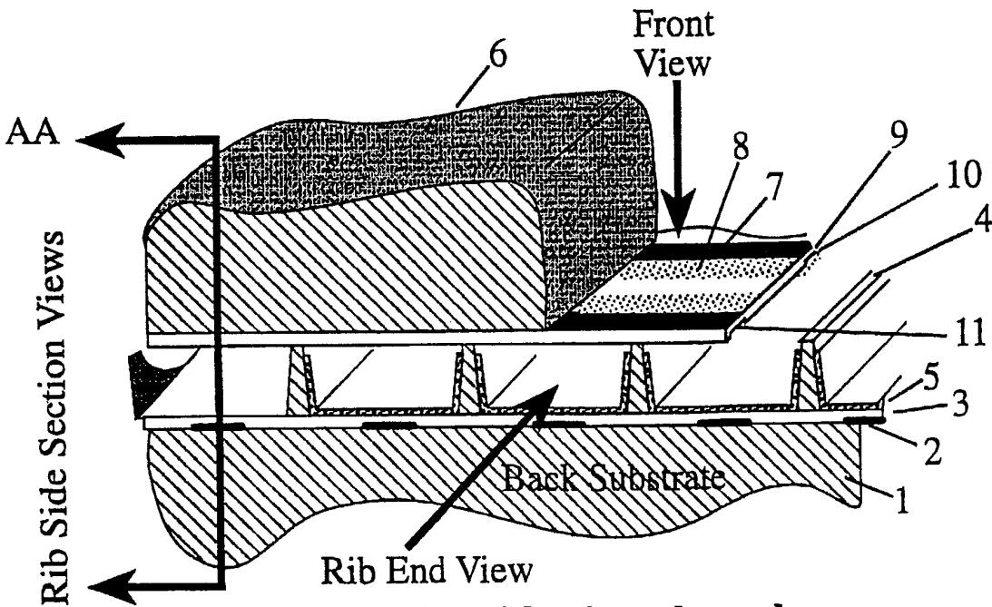
Fig. 2 PDP device with micro-channels
