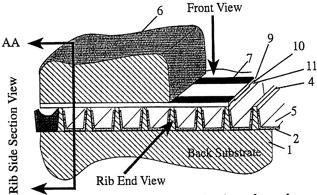
Fig. 1 MOG PDP device with micro-channels
