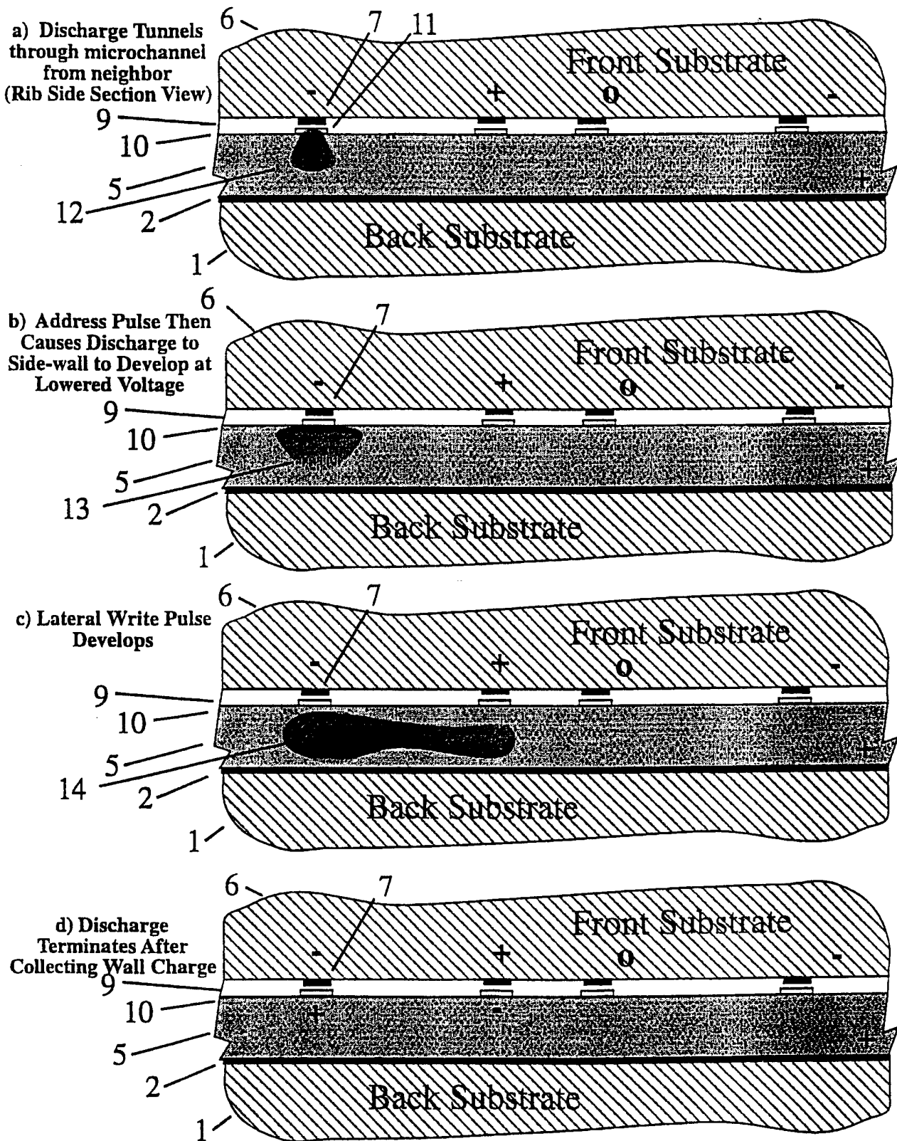
Fig. 5 Tunnel Addressing Sequence
