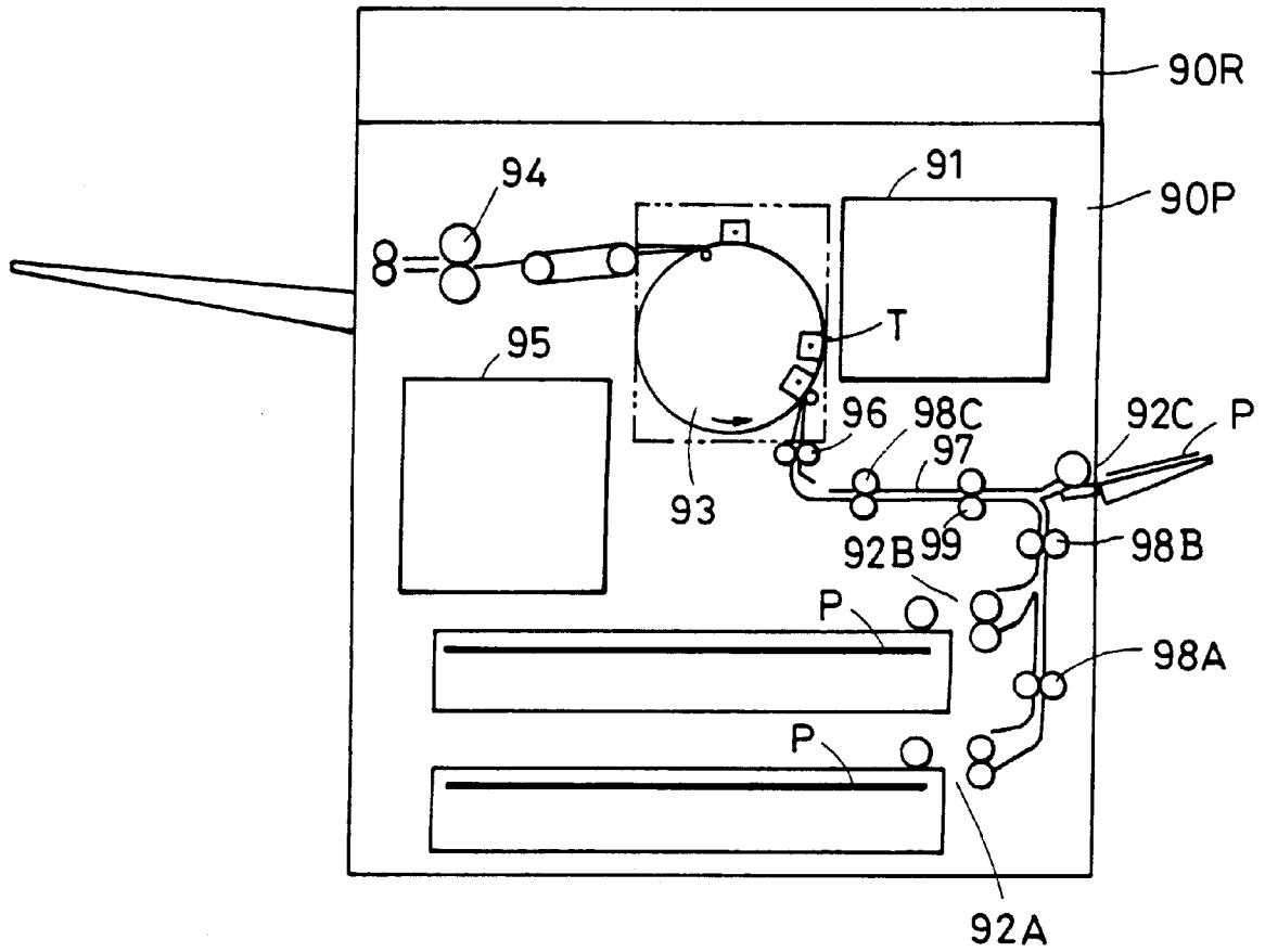
FIG. 7 PRIOR ART
