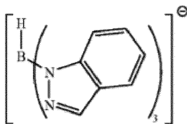
Chemical Formula 5-1-1
