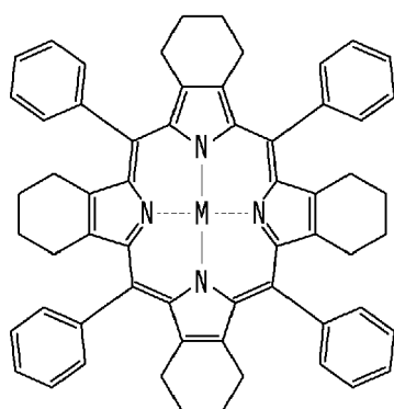
Chemical Formula 1-8
