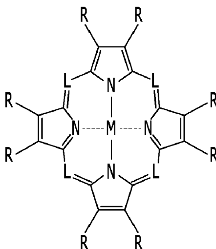
Chemical Formula 1
