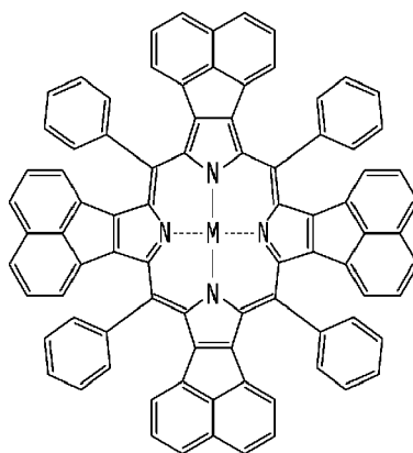
Chemical Formula 1-4
