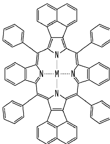
Chemical Formula 1-5
