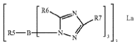
Chemical Formula 7
