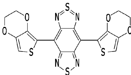
Chemical Formula 4
