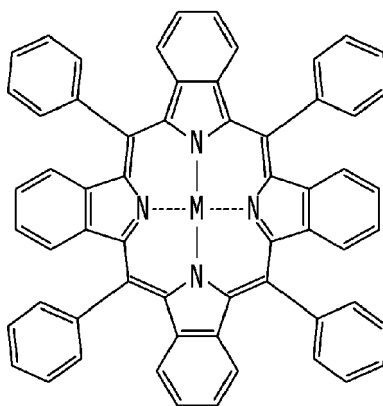
Chemical Formula 1-1
