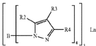
Chemical Formula 8
