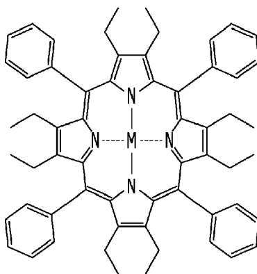
Chemical Formula 1-9
