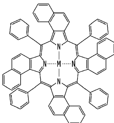
Chemical Formula 1-3
