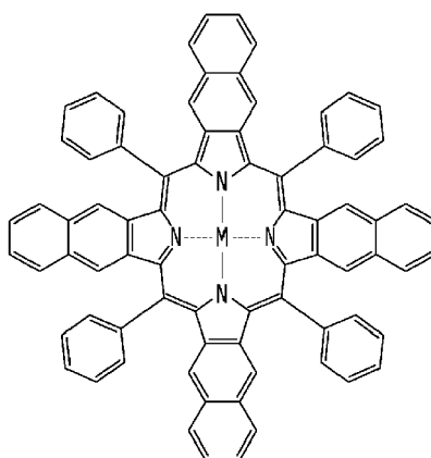
Chemical Formula 1-6
