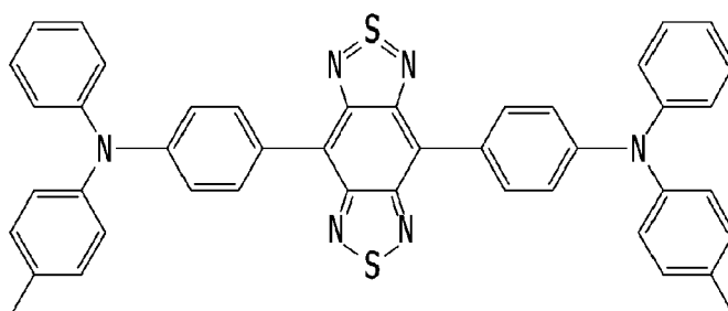
Chemical Formula 2
