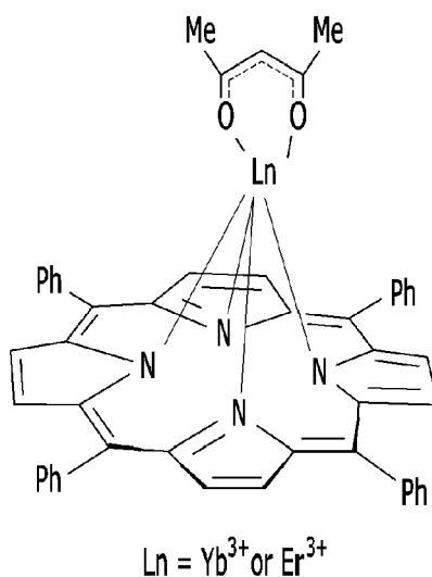
Chemical Formula 10
