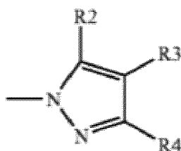
Chemical Formula 5-1
