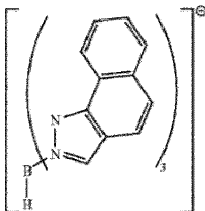
Chemical Formula 5-2-1
