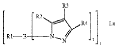
Chemical Formula 6
