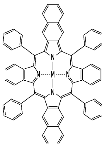
Chemical Formula 1-2
