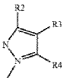
Chemical Formula 5-2
