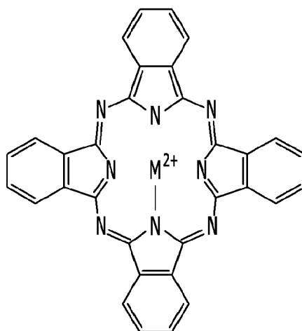
Chemical Formula 1-10
