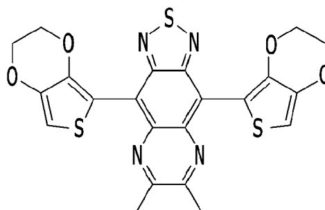
Chemical Formula 3
