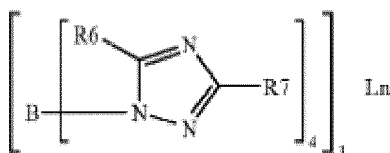
Chemical Formula 9
