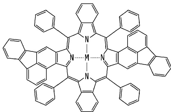
Chemical Formula 1-7
