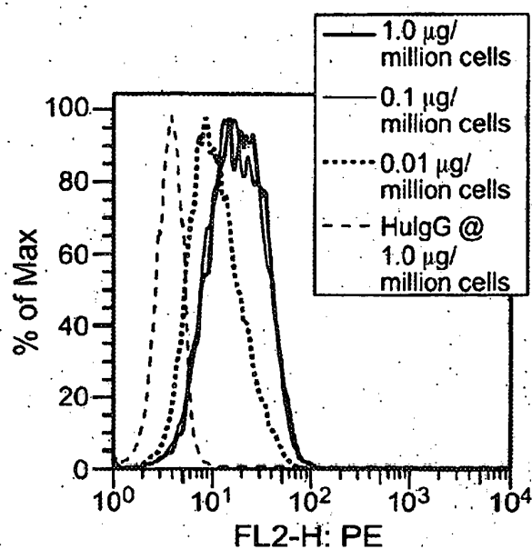
Binding of Thio MA79b.v18-HC (A118C)-MC-MMAF to BJAB-luc8
