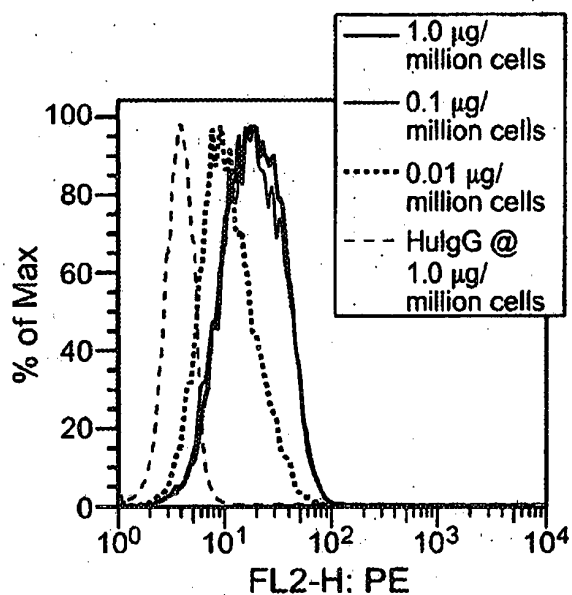
Binding of Thio MA79b.v18-HC (A118C)-MCvcPAB-MMAE to BJAB-luc8
