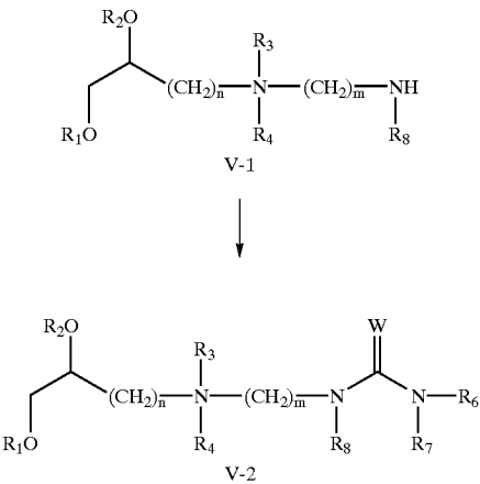
Scheme V
