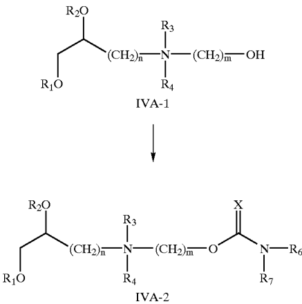
Scheme IV
