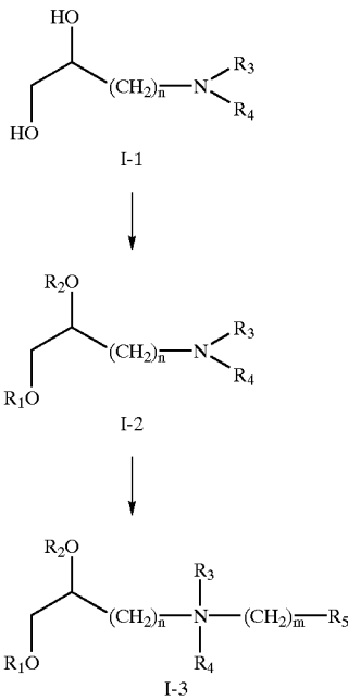
Scheme I
