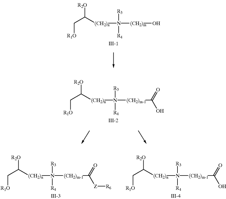
Scheme III
