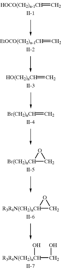
Scheme II
