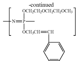
Polyphosphazene
