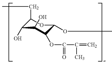
Methacrylate-Modified Dextran
