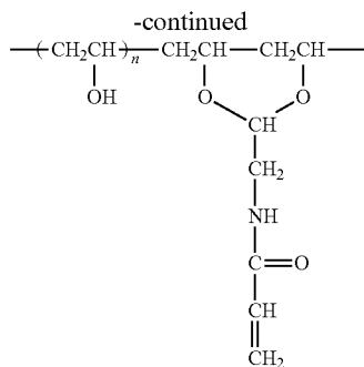
Acrylic Modified PVA
