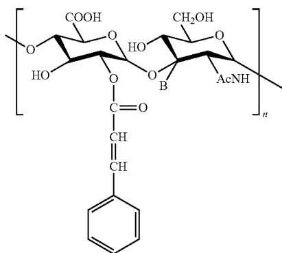
Commutated Hyaluronic Acid
