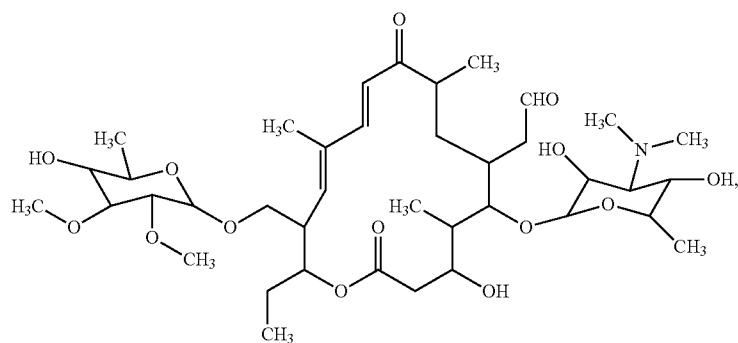
tylosin B (also known as desmycocin)
