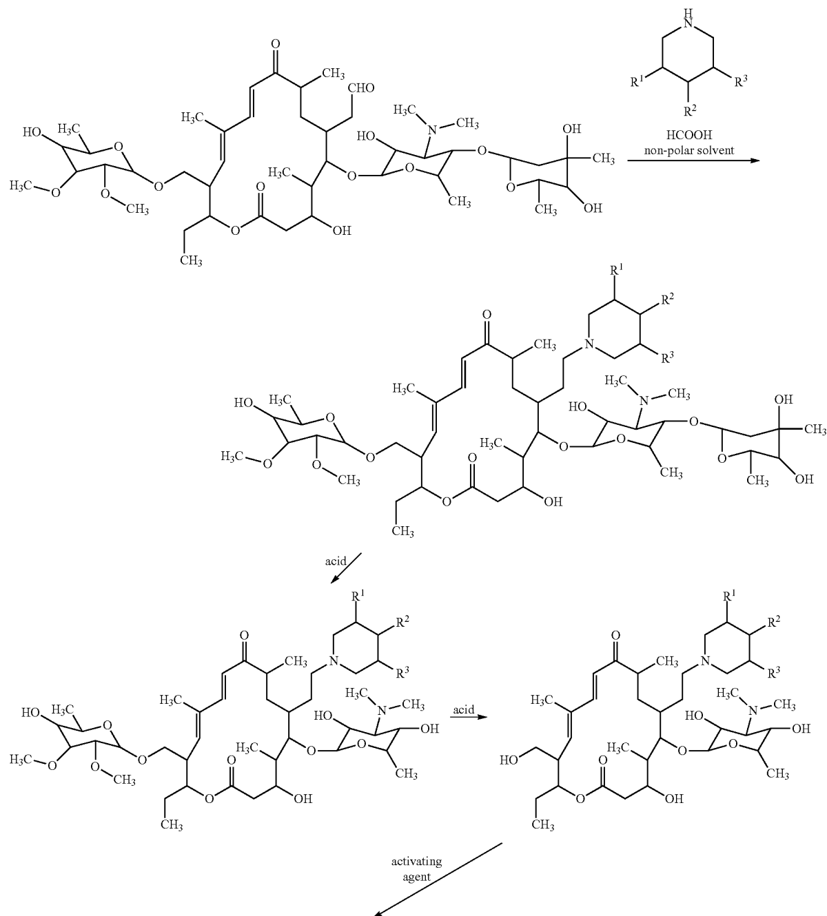
Scheme I
