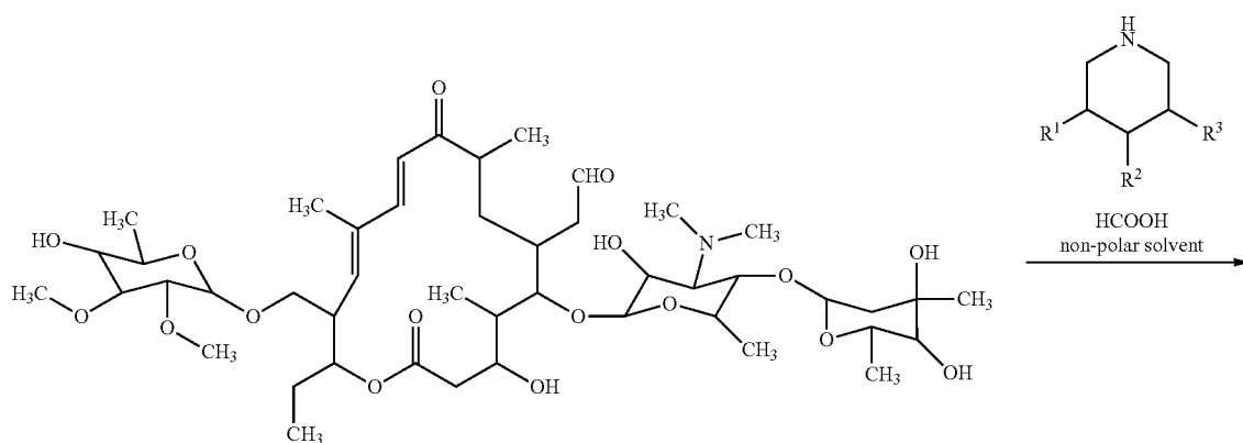
Scheme III
