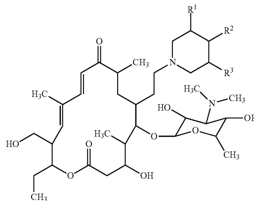
23-hydroxyl-20-piperidinyl-5-O-mycaminosyl-tylonolide compound
