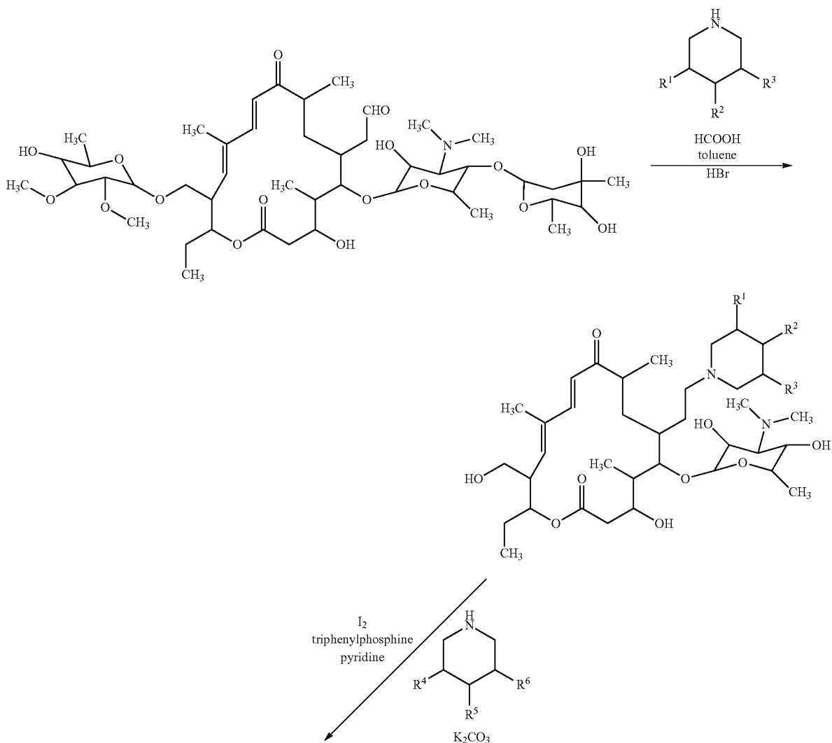
Scheme V
