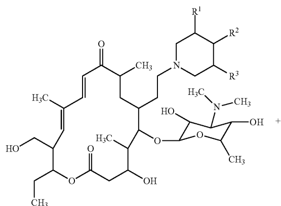
23-hydroxyl-20-piperidinyl-5-O-mycaminosyl-tylonolide compound
