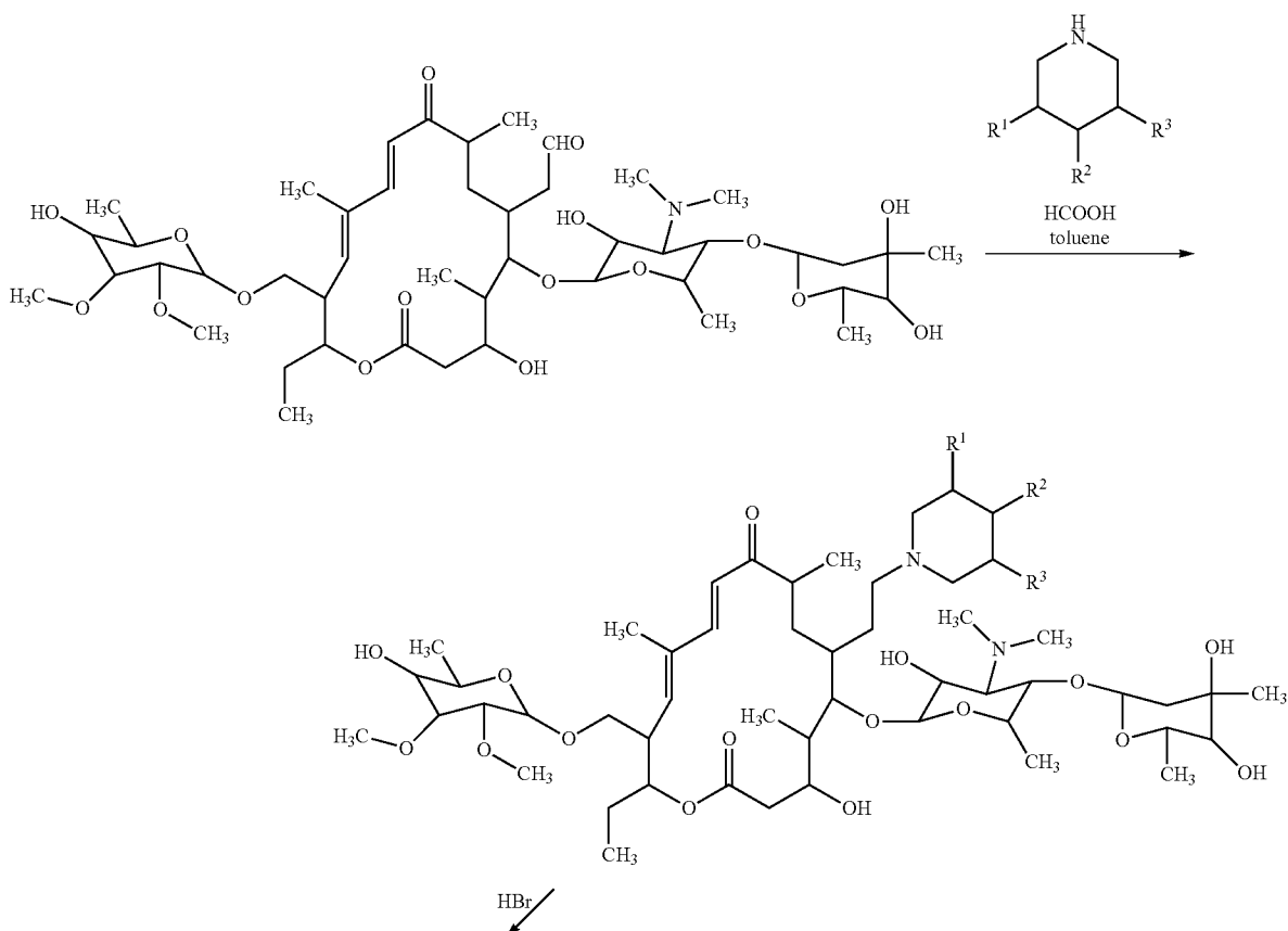
Scheme II
