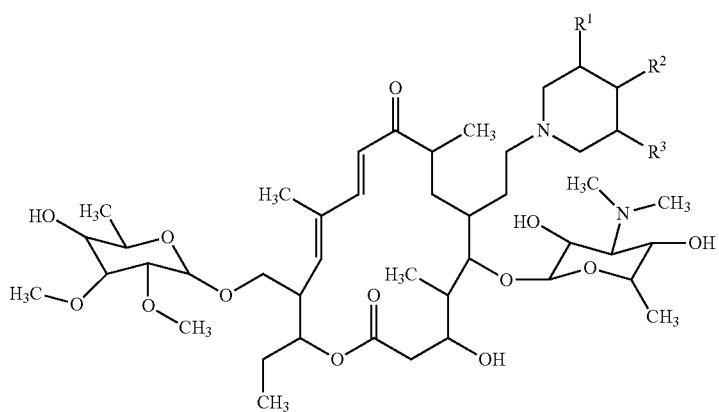
23-O-mycinosyl-20-piperidinyl-5-O-mycaminosyl-tylonolide compound
