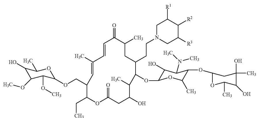
20-piperidinyl-tylosin compound
