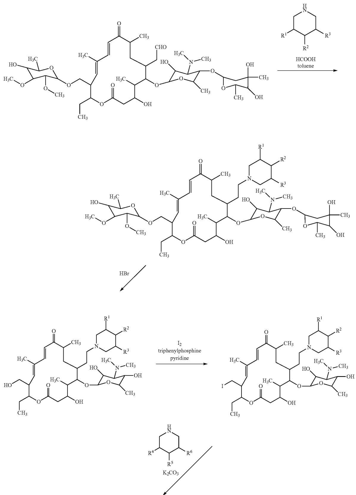
Scheme IV
