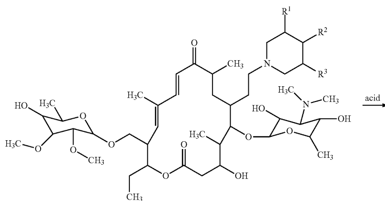
23-O-mycinosyl-20-piperidinyl-5-O-mycaminosyl-tylonolide compound
