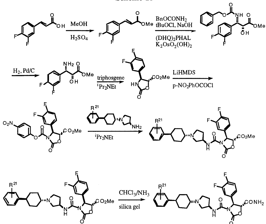
Scheme 15
