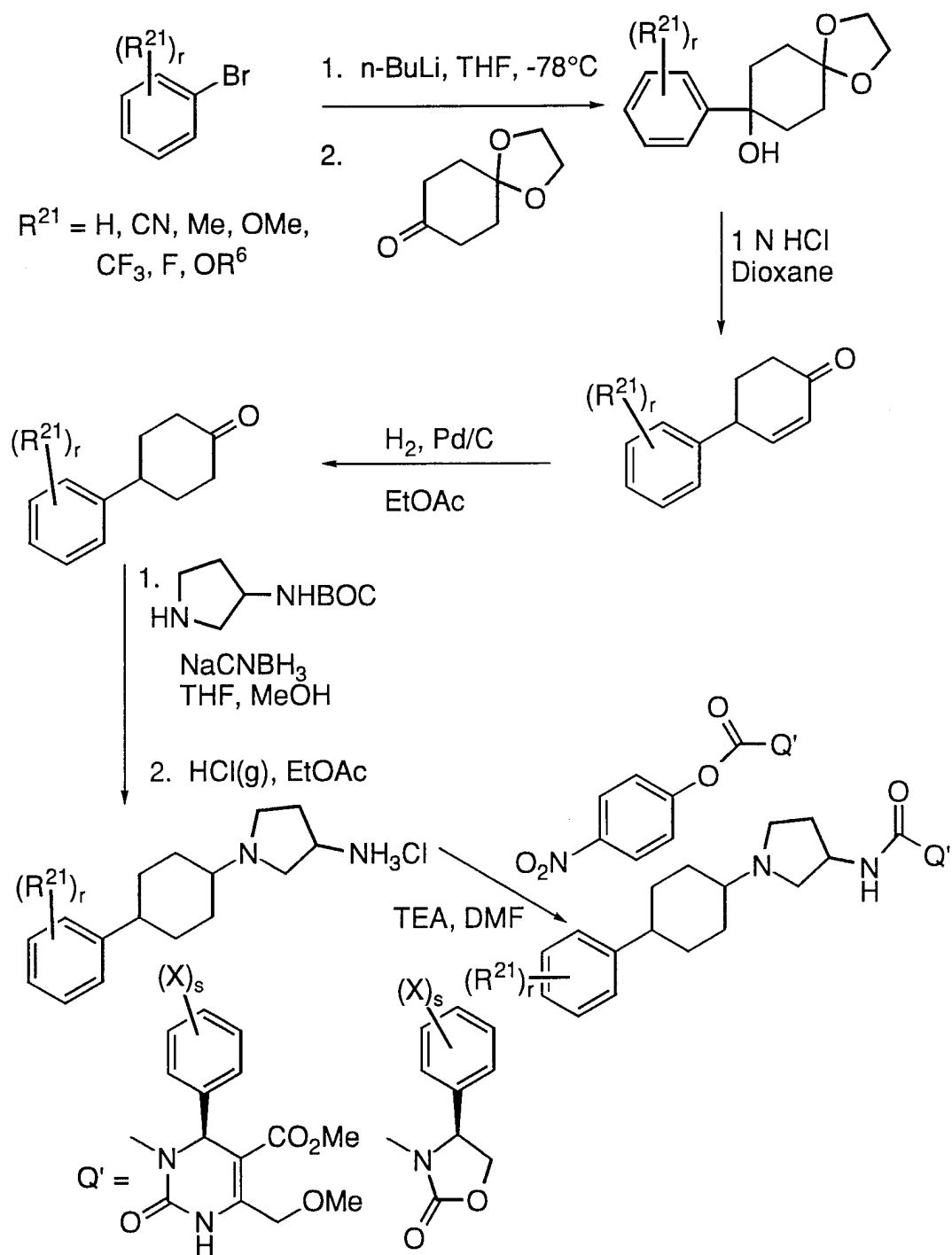
Scheme 10
