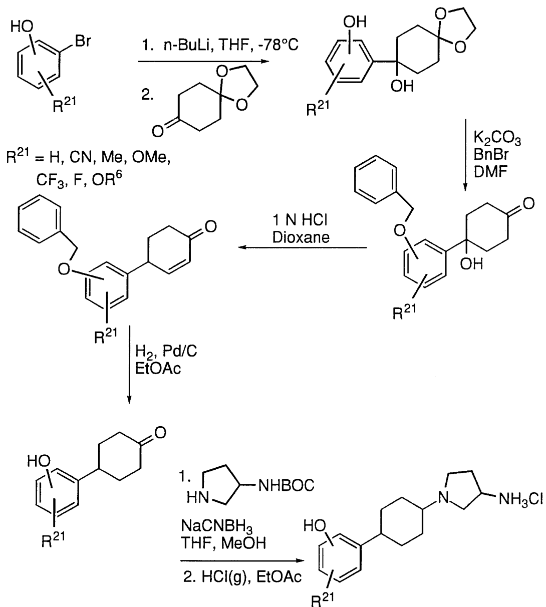
Scheme 13
