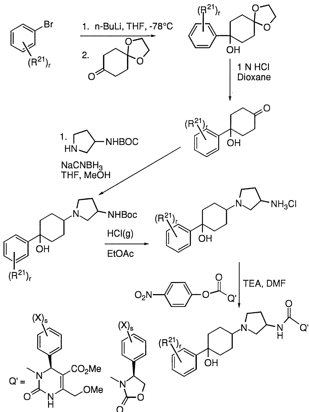
Scheme 12
