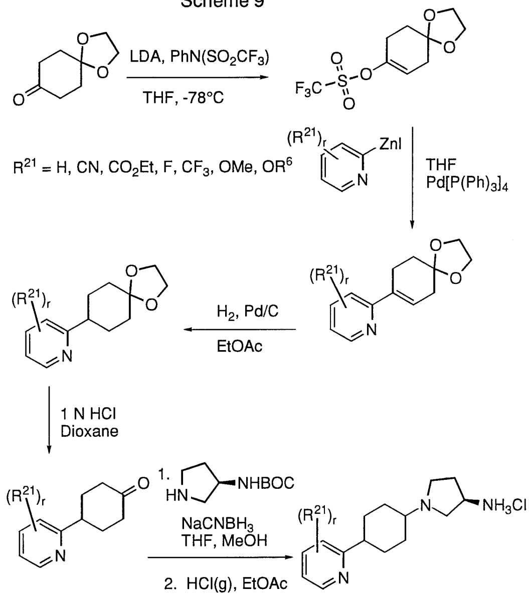
Scheme 9
