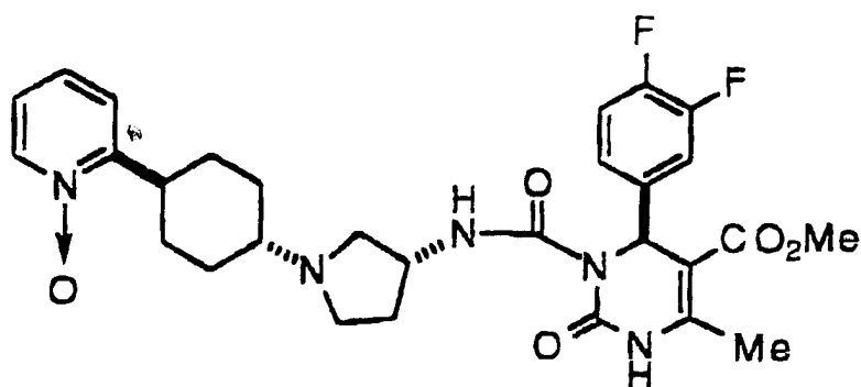
Compound C:
