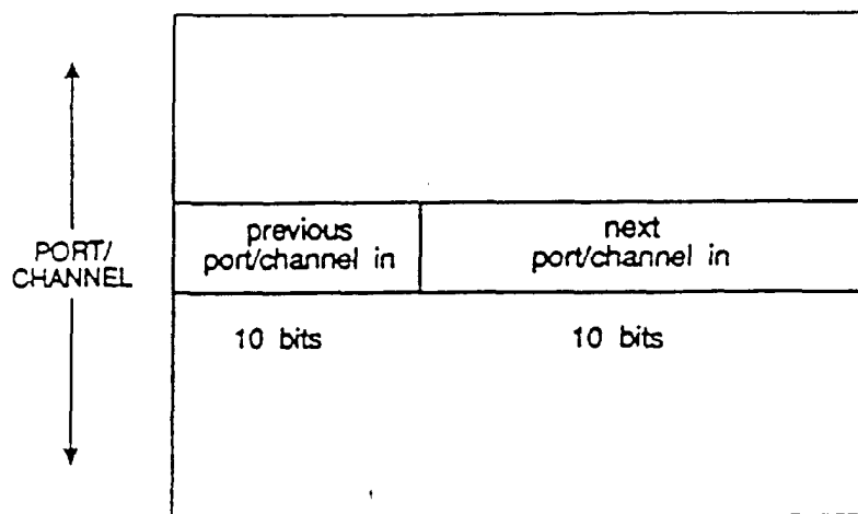
NEXT CHANNEL IN LINK LIST TABLE
