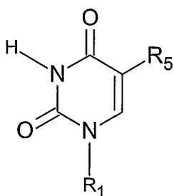
Figure 1g, Uracil, U
