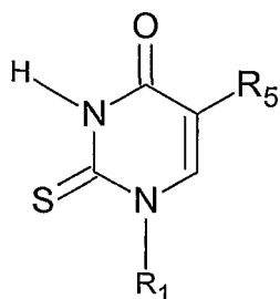
Figure 1h, 2-ThioUracil, U2s
