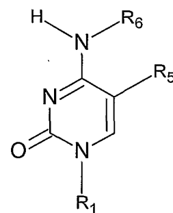
Figure 1j, Cytosine, C
