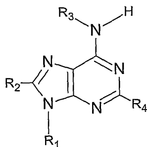
Figure 1a, Adenine, A
