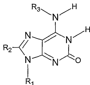
Figure 1m, isoGuanine, isoG
