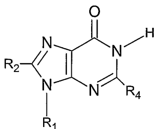
Figure 1f, Inosine, I
