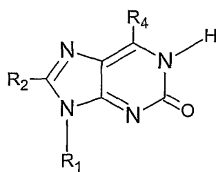
Figure 1o, 2-oxoPurine, Pu-2o
