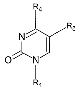
Figure 1k, 2-oxo-Pyrimidine, Py-2o
