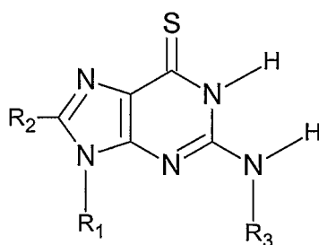
Figure 1e, ThioGuanine, Gs
