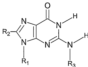
Figure 1d, Guanine, G
