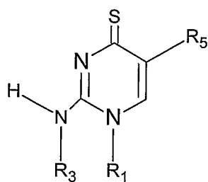
Figure 1q, isothioCytosine, isoCs
