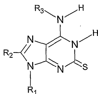
Figure 1n, isothioGuanine, isoGs
