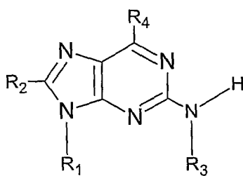
Figure 1b, isoAdenine, isoA
