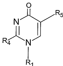
Figure 1r, 4-oxoPyrimidine, Py-4o
