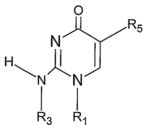
Figure 1p, isoCytosine, isoC
