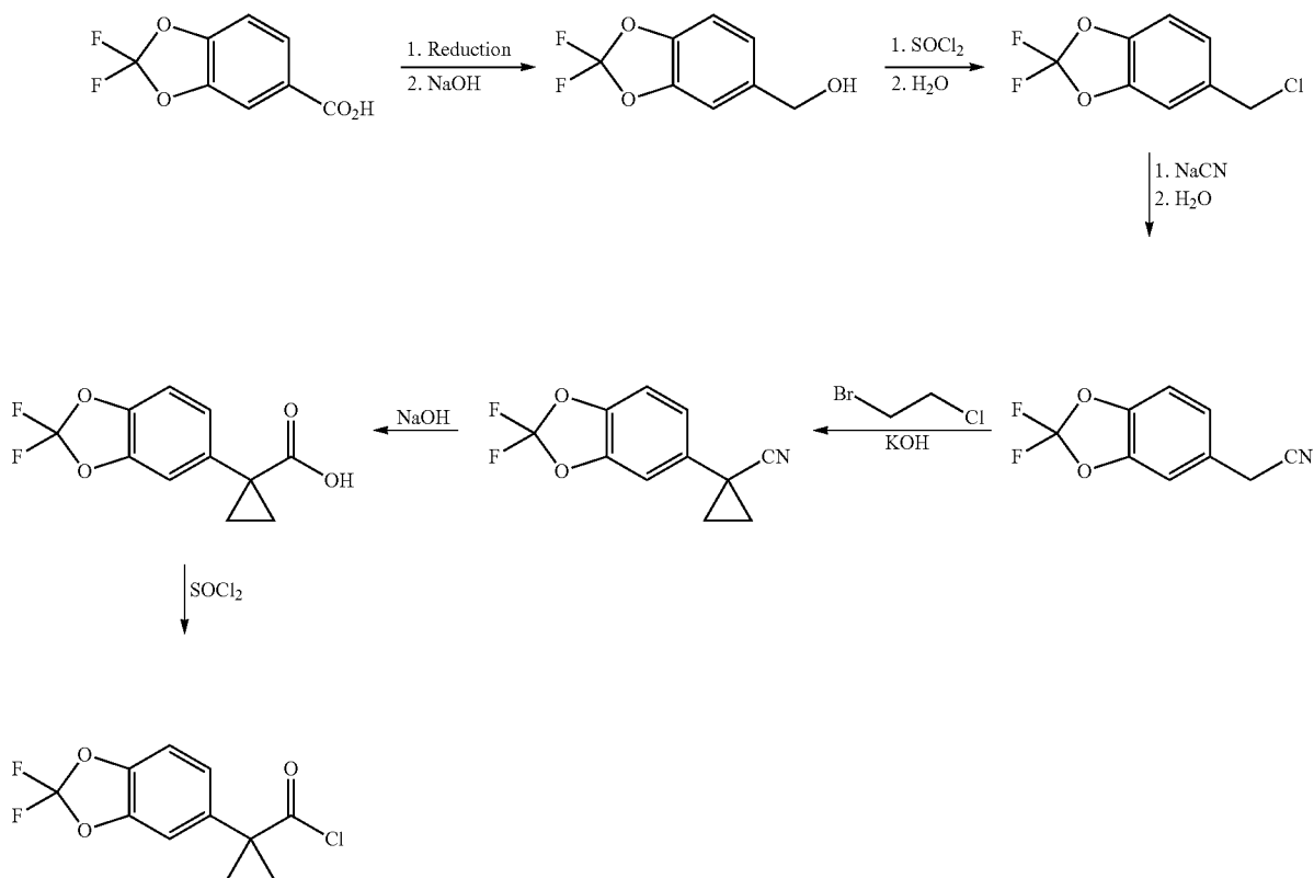
Scheme 1. Synthesis of the acid chloride moiety.
