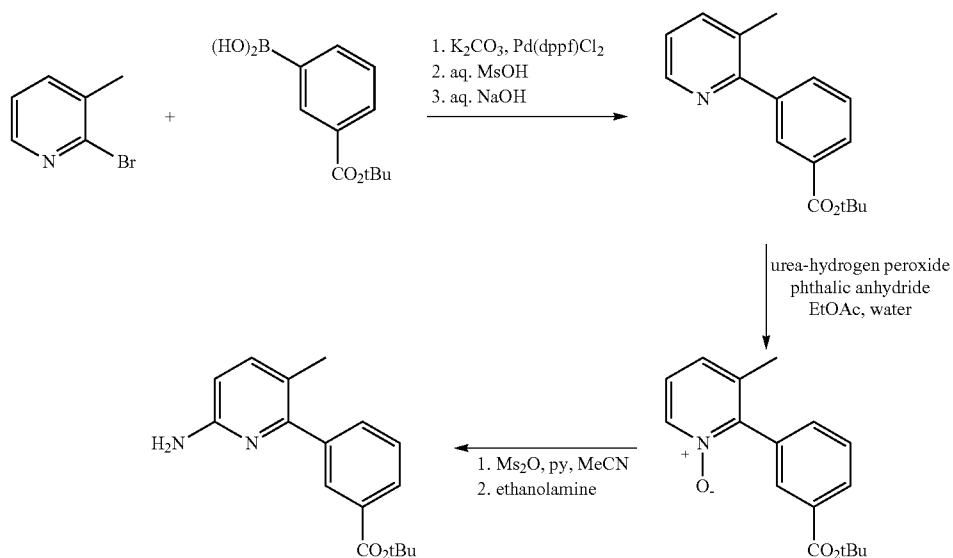
Scheme 3. Synthesis of the amine moiety.
