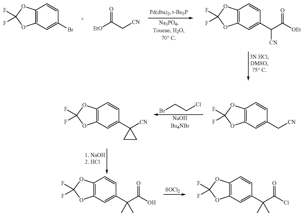
Scheme 2. Alternative synthesis of the acid chloride moiety.
