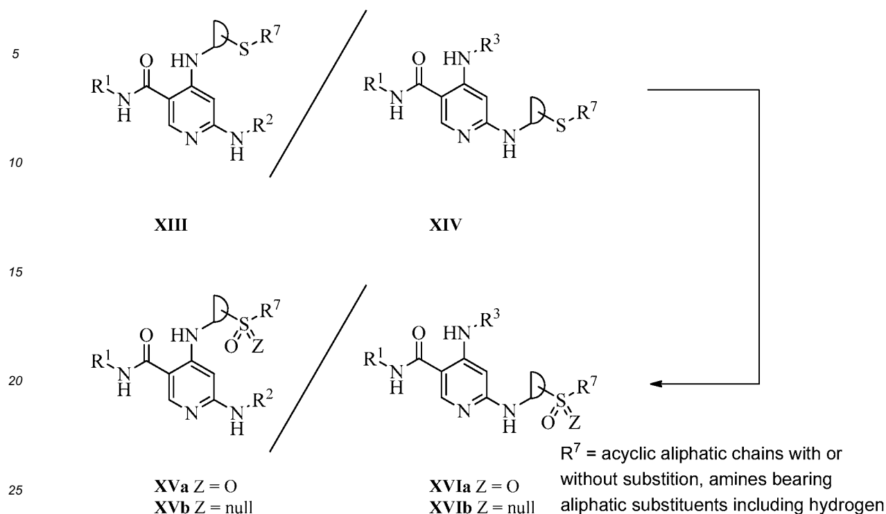
Scheme 5. Oxidation of pendant sulfides XIII and XIV
