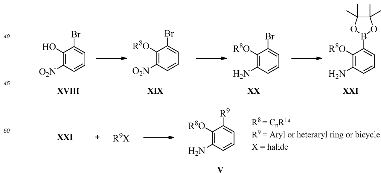
Scheme 6. Synthesis of anilines V
