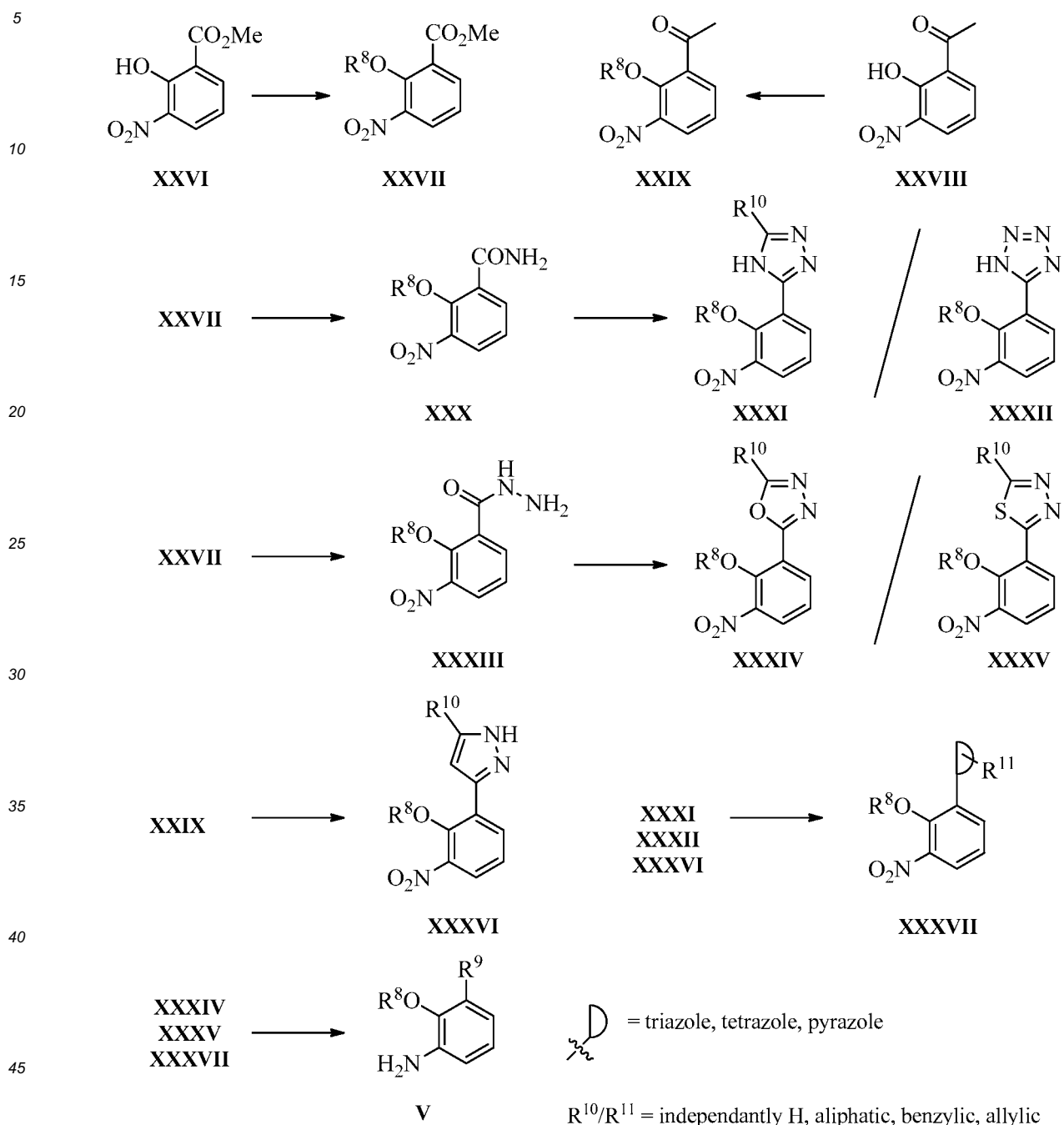
Scheme 8. Alternate synthesis of anilines V
