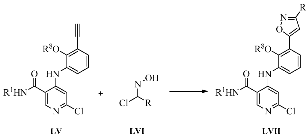
Scheme 13. Synthesis of LVII
