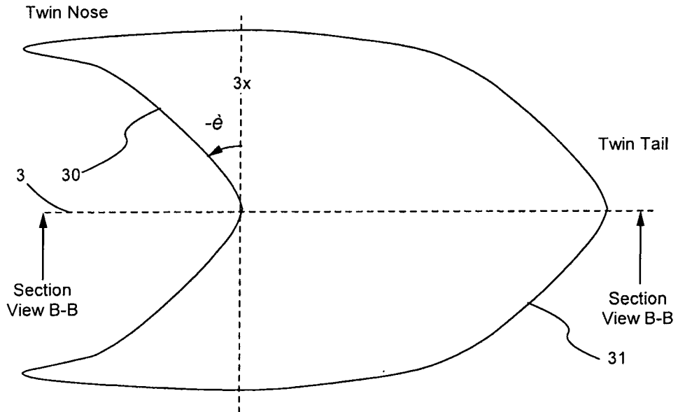
Figure 2b Plan
