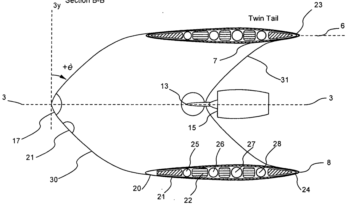
Figure 2a Elevation Section B-B
