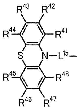
General Formula (6)
