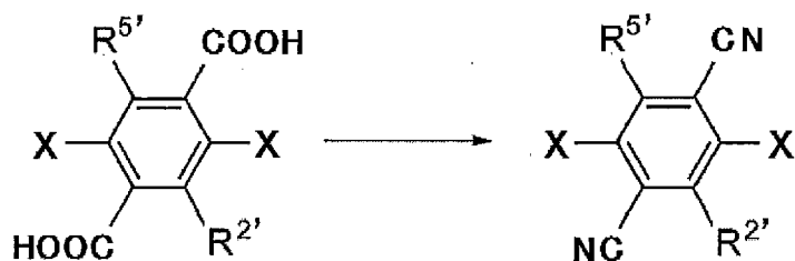
Compound A
