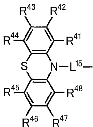
General Formula (6)
