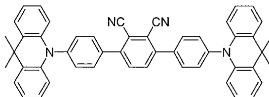
Compound 16
