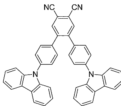
Compound 18
