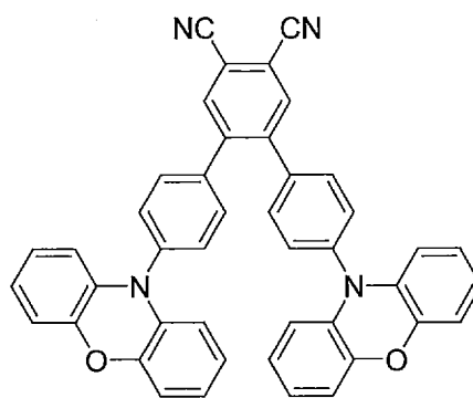
Compound 20
