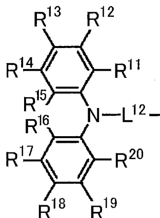
General Formula (2)
