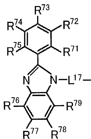
General Formula (7)
