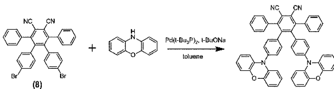
Compound 31
