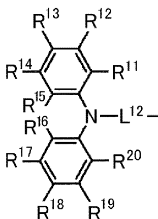
General Formula (2)
