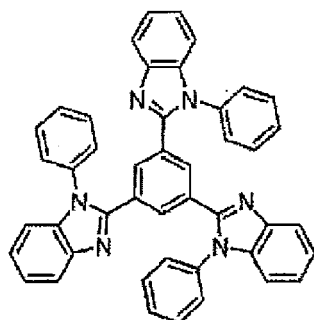
TPBi
