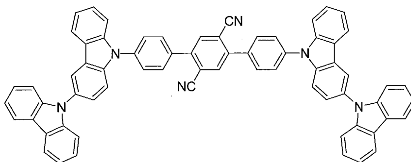
Compound 5
