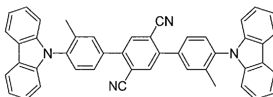
Compound 4
