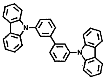
mCBP
