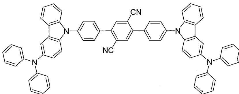
Compound 6
