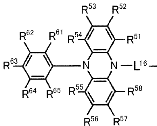
General Formula (6)
