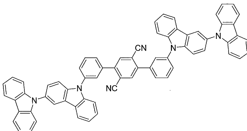
Compound 13
