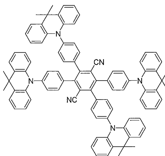
Compound 8
