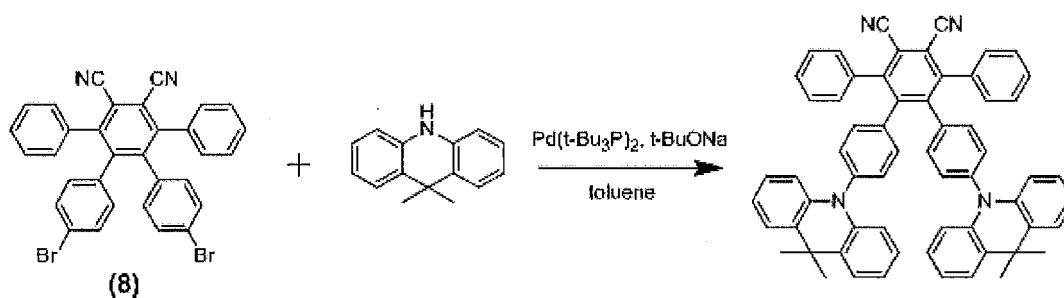
Compound 30
