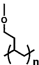
Formula (11)
