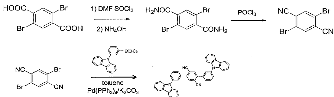
Compound 3
