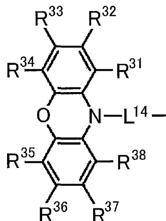
General Formula (4)
