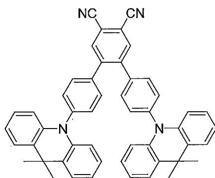
Compound 19
