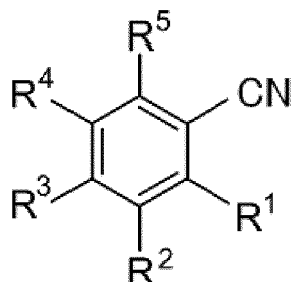
General Formula (1)
