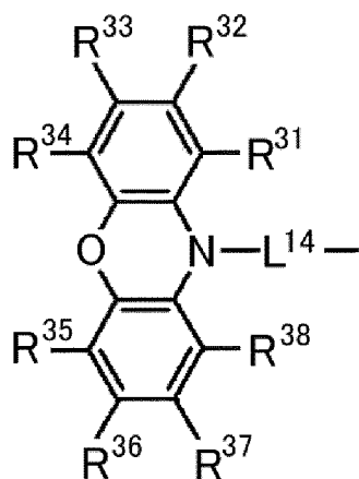
General Formula (5)
