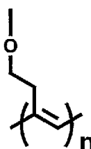
Formula (12)
