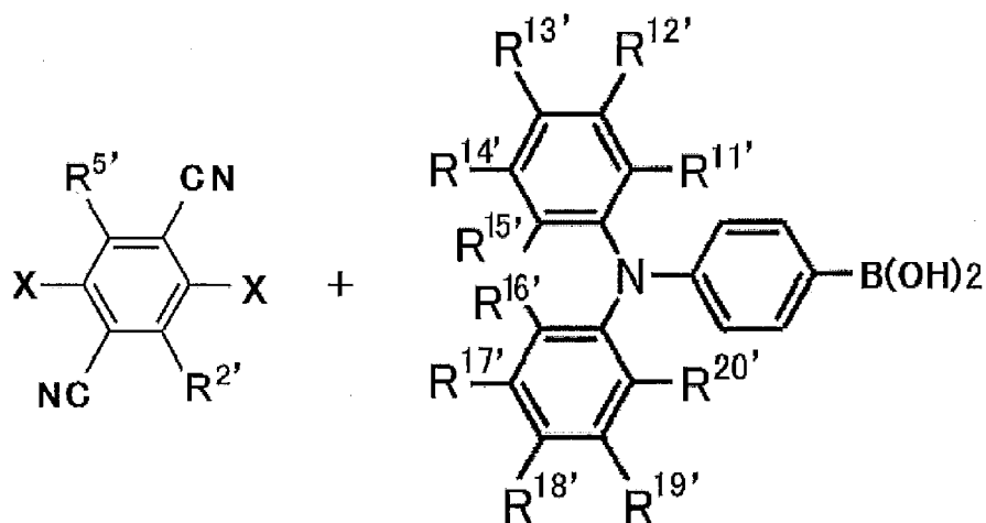
Compound A
