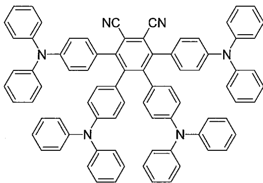
Compound 25
