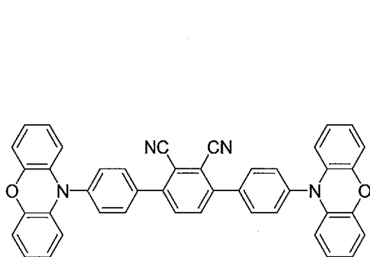
Compound 17
